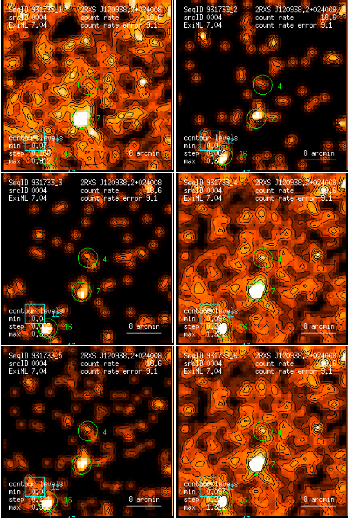
Figure 4: RASS 931733: detection 0004: band rate images, Gaussian filter: (1) PSPC channels 11 – 41, (2) 52 – 90, (3) 91 – 201, (4) 11 – 235, (5) 52 – 201, (6) 11 – 201. Broad band rates in counts/ks. Band rate contour levels in counts/ks/arcmin 2 .
