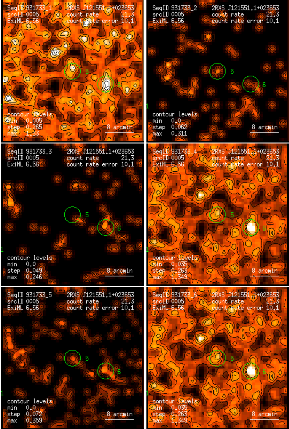
Figure 5: RASS 931733: detection 0005: band rate images, Gaussian filter: (1) PSPC channels 11 – 41, (2) 52 – 90, (3) 91 – 201, (4) 11 – 235, (5) 52 – 201, (6) 11 – 201. Broad band rates in counts/ks. Band rate contour levels in counts/ks/arcmin 2 .
