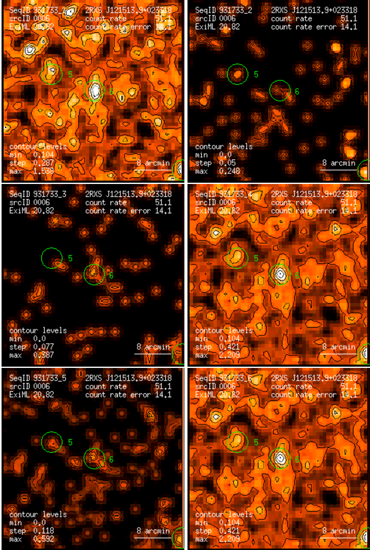
Figure 6: RASS 931733: detection 0006: band rate images, Gaussian filter: (1) PSPC channels 11 – 41, (2) 52 – 90, (3) 91 – 201, (4) 11 – 235, (5) 52 – 201, (6) 11 – 201. Broad band rates in counts/ks. Band rate contour levels in counts/ks/arcmin 2 .
