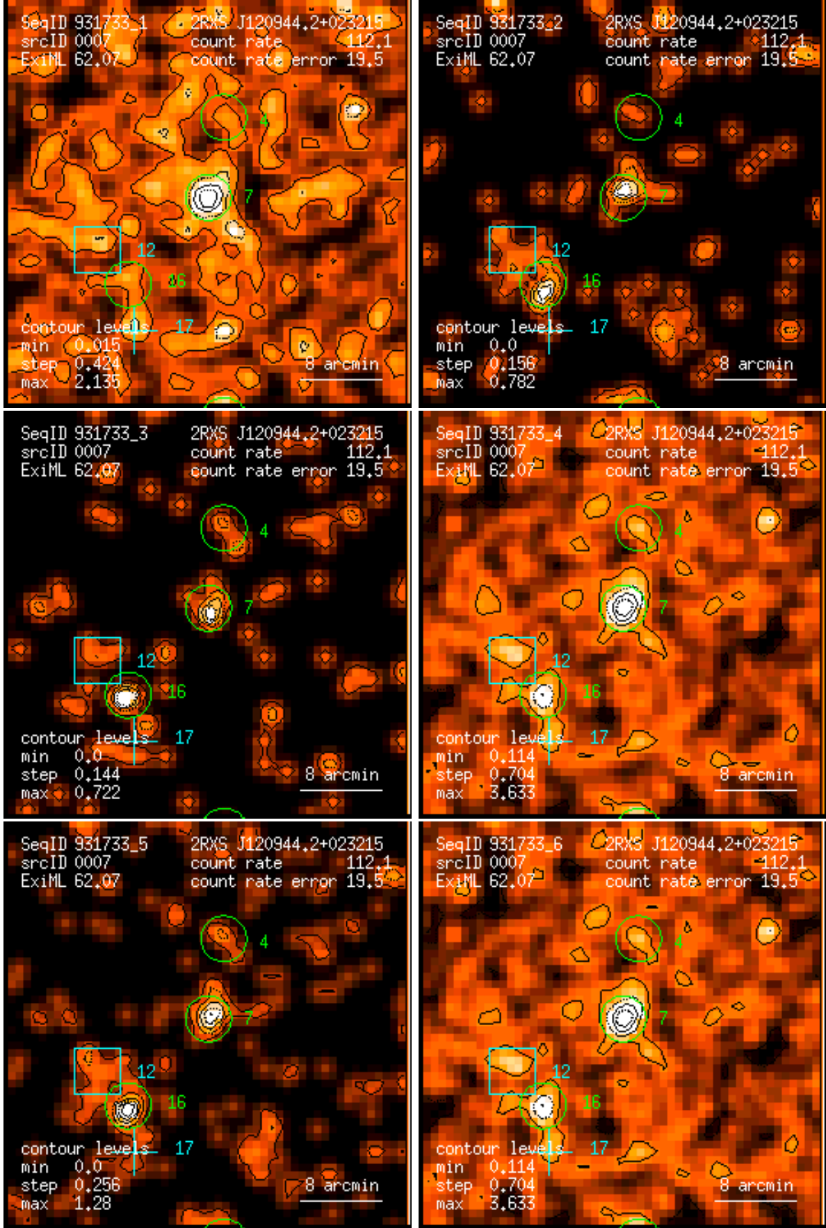
Figure 7: RASS 931733: detection 0007: band rate images, Gaussian filter: (1) PSPC channels 11 – 41, (2) 52 – 90, (3) 91 – 201, (4) 11 – 235, (5) 52 – 201, (6) 11 – 201. Broad band rates in counts/ks. Band rate contour levels in counts/ks/arcmin 2 .
