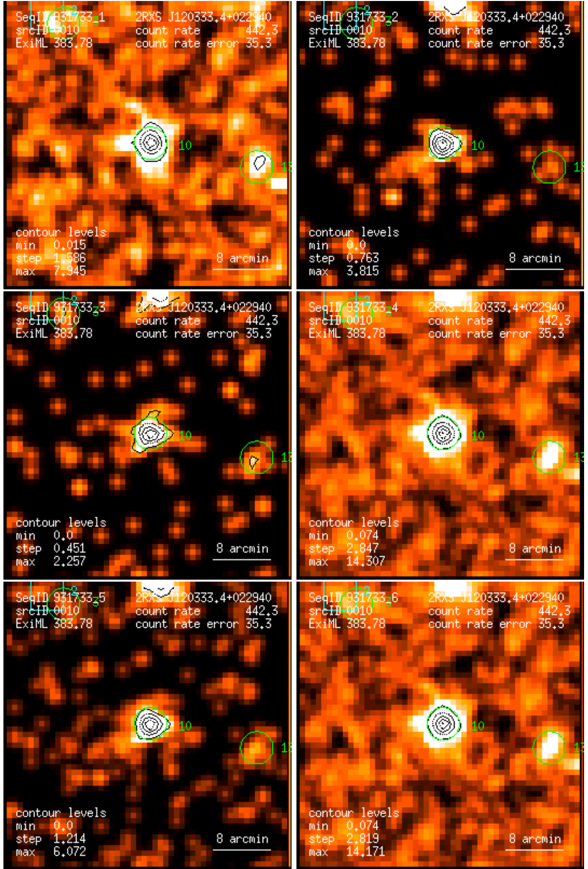
Figure 10: RASS 931733: detection 0010: band rate images, Gaussian filter: (1) PSPC channels 11 – 41, (2) 52 – 90, (3) 91 – 201, (4) 11 – 235, (5) 52 – 201, (6) 11 – 201. Broad band rates in counts/ks. Band rate contour levels in counts/ks/arcmin 2 .
