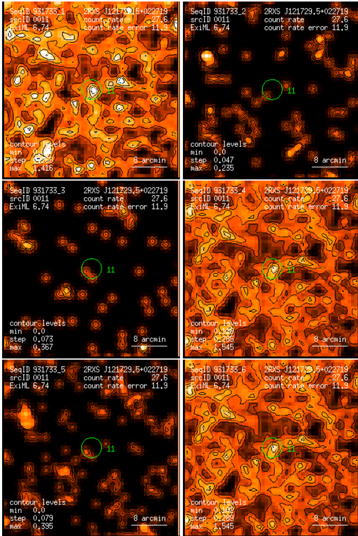
Figure 11: RASS 931733: detection 0011: band rate images, Gaussian filter: (1) PSPC channels 11 – 41, (2) 52 – 90, (3) 91 – 201, (4) 11 – 235, (5) 52 – 201, (6) 11 – 201. Broad band rates in counts/ks. Band rate contour levels in counts/ks/arcmin 2 .
