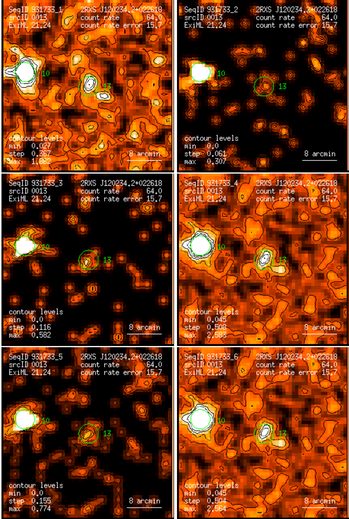
Figure 13: RASS 931733: detection 0013: band rate images, Gaussian filter: (1) PSPC channels 11 – 41, (2) 52 – 90, (3) 91 – 201, (4) 11 – 235, (5) 52 – 201, (6) 11 – 201. Broad band rates in counts/ks. Band rate contour levels in counts/ks/arcmin 2 .
