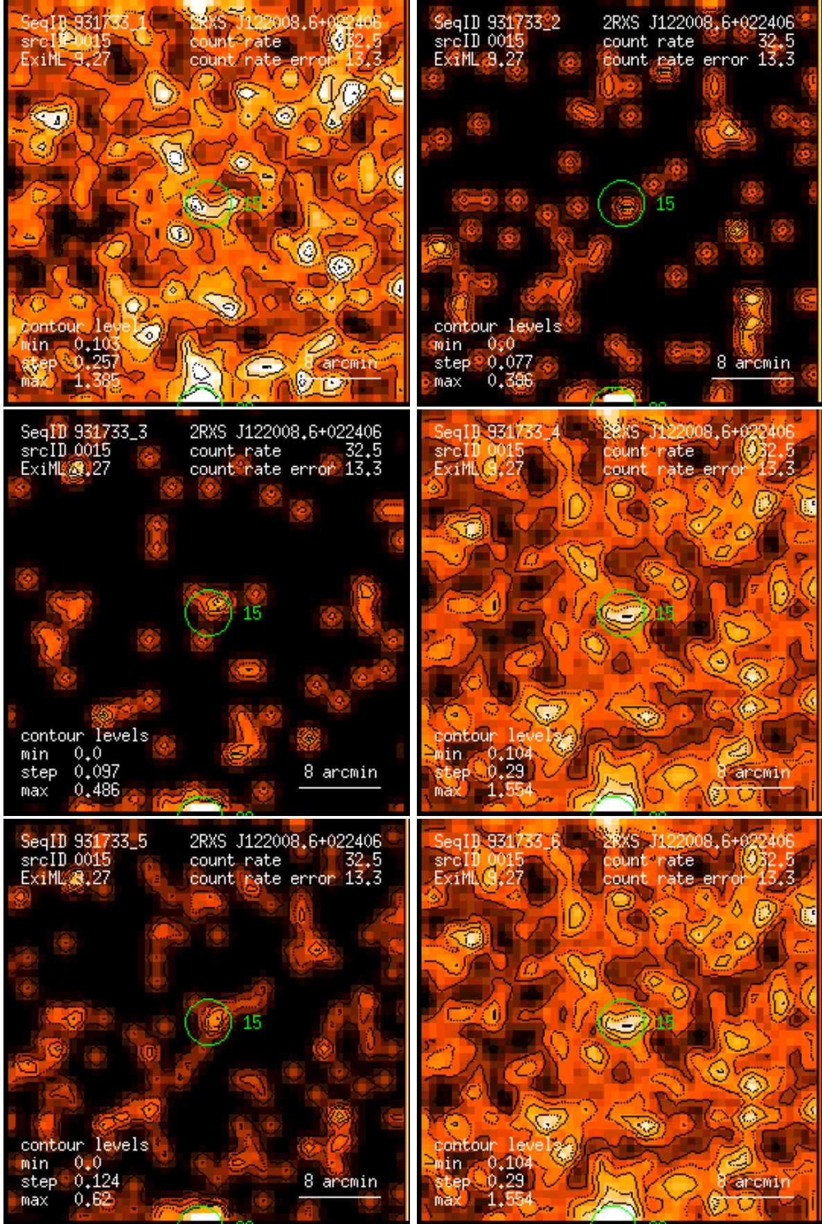
Figure 15: RASS 931733: detection 0015: band rate images, Gaussian filter: (1) PSPC channels 11 – 41, (2) 52 – 90, (3) 91 – 201, (4) 11 – 235, (5) 52 – 201, (6) 11 – 201. Broad band rates in counts/ks. Band rate contour levels in counts/ks/arcmin 2 .
