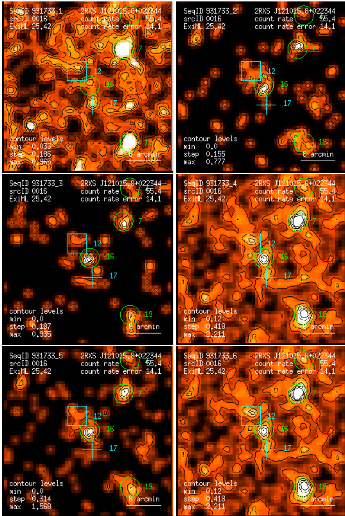
Figure 16: RASS 931733: detection 0016: band rate images, Gaussian filter: (1) PSPC channels 11 – 41, (2) 52 – 90, (3) 91 – 201, (4) 11 – 235, (5) 52 – 201, (6) 11 – 201. Broad band rates in counts/ks. Band rate contour levels in counts/ks/arcmin 2 .
