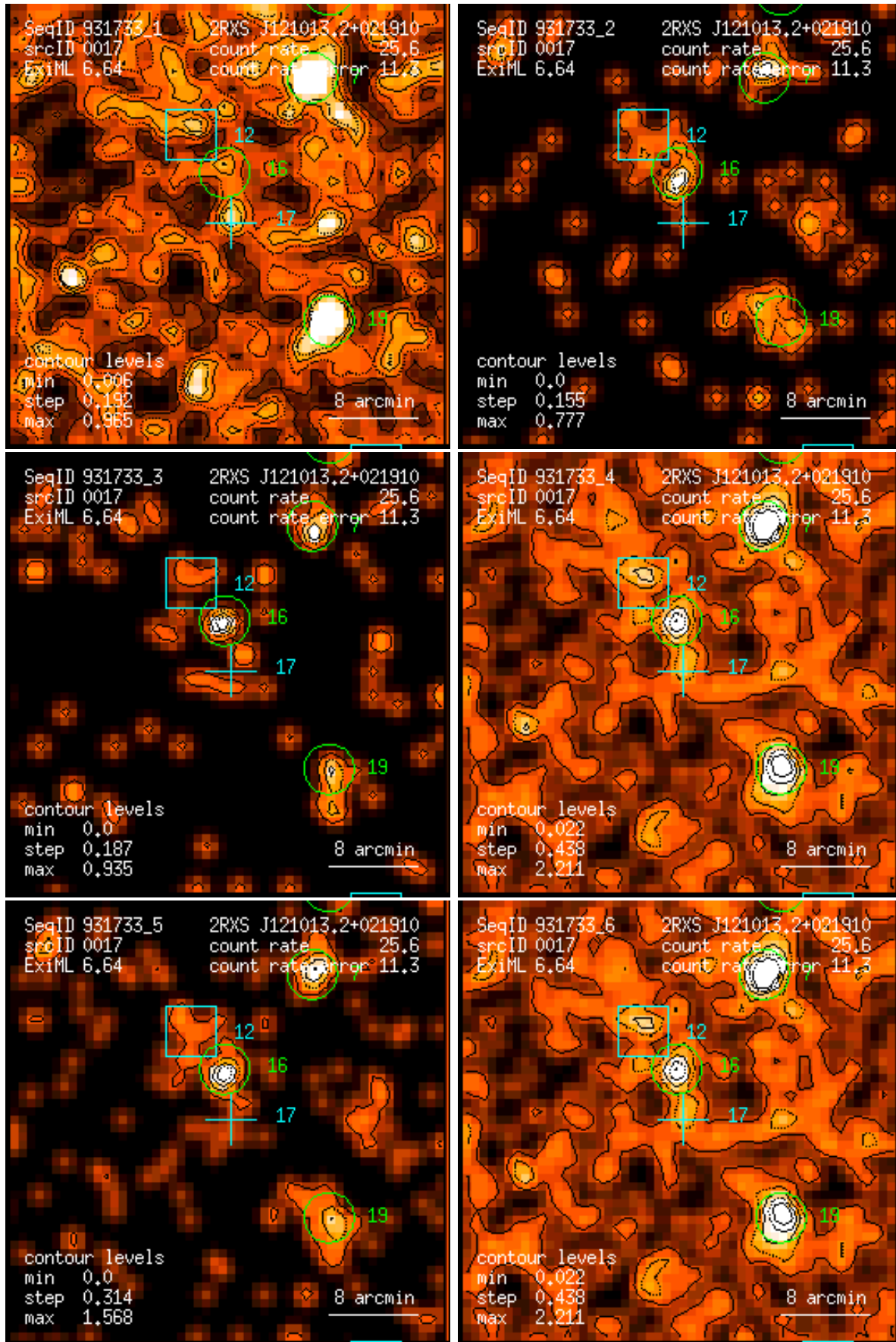
Figure 17: RASS 931733: detection 0017: band rate images, Gaussian filter: (1) PSPC channels 11 – 41, (2) 52 – 90, (3) 91 – 201, (4) 11 – 235, (5) 52 – 201, (6) 11 – 201. Broad band rates in counts/ks. Band rate contour levels in counts/ks/arcmin 2 .
