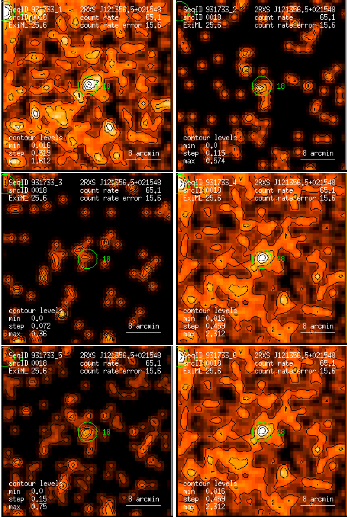
Figure 18: RASS 931733: detection 0018: band rate images, Gaussian filter: (1) PSPC channels 11 – 41, (2) 52 – 90, (3) 91 – 201, (4) 11 – 235, (5) 52 – 201, (6) 11 – 201. Broad band rates in counts/ks. Band rate contour levels in counts/ks/arcmin 2 .
