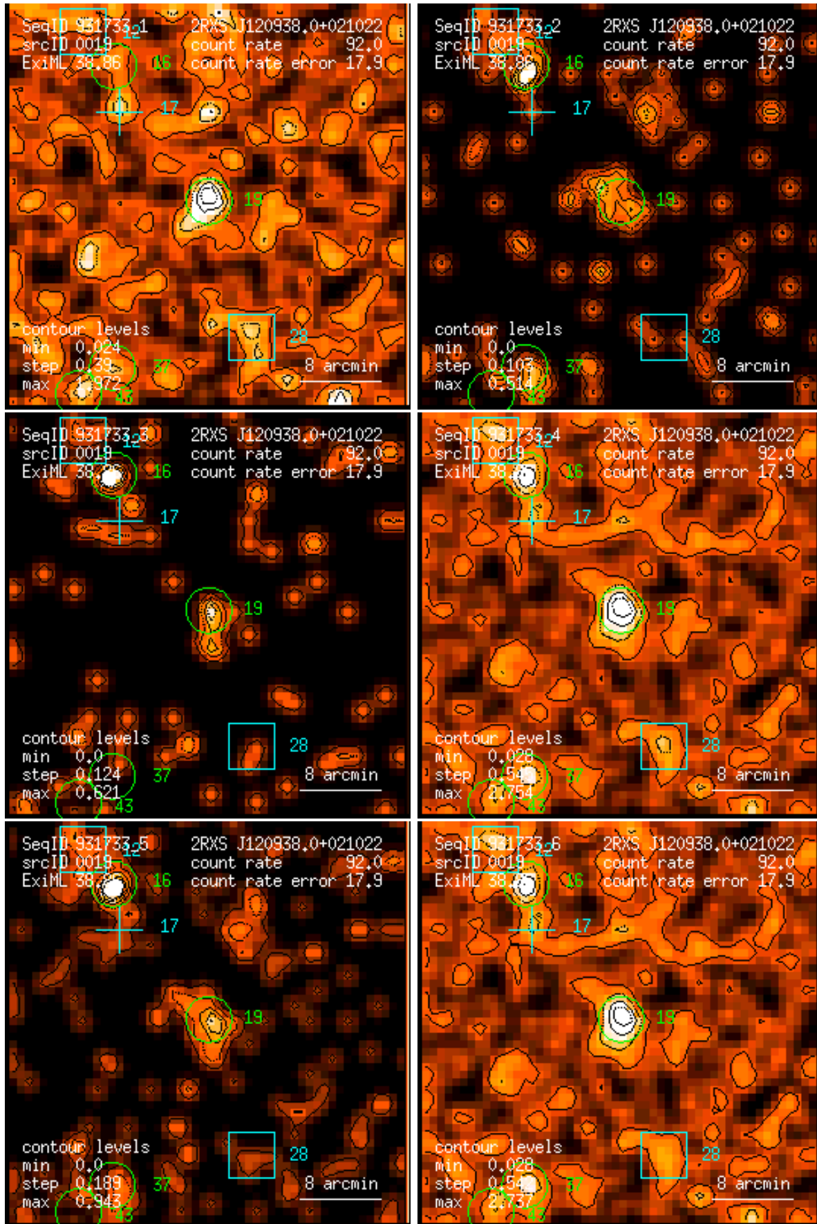
Figure 19: RASS 931733: detection 0019: band rate images, Gaussian filter: (1) PSPC channels 11 – 41, (2) 52 – 90, (3) 91 – 201, (4) 11 – 235, (5) 52 – 201, (6) 11 – 201. Broad band rates in counts/ks. Band rate contour levels in counts/ks/arcmin 2 .
