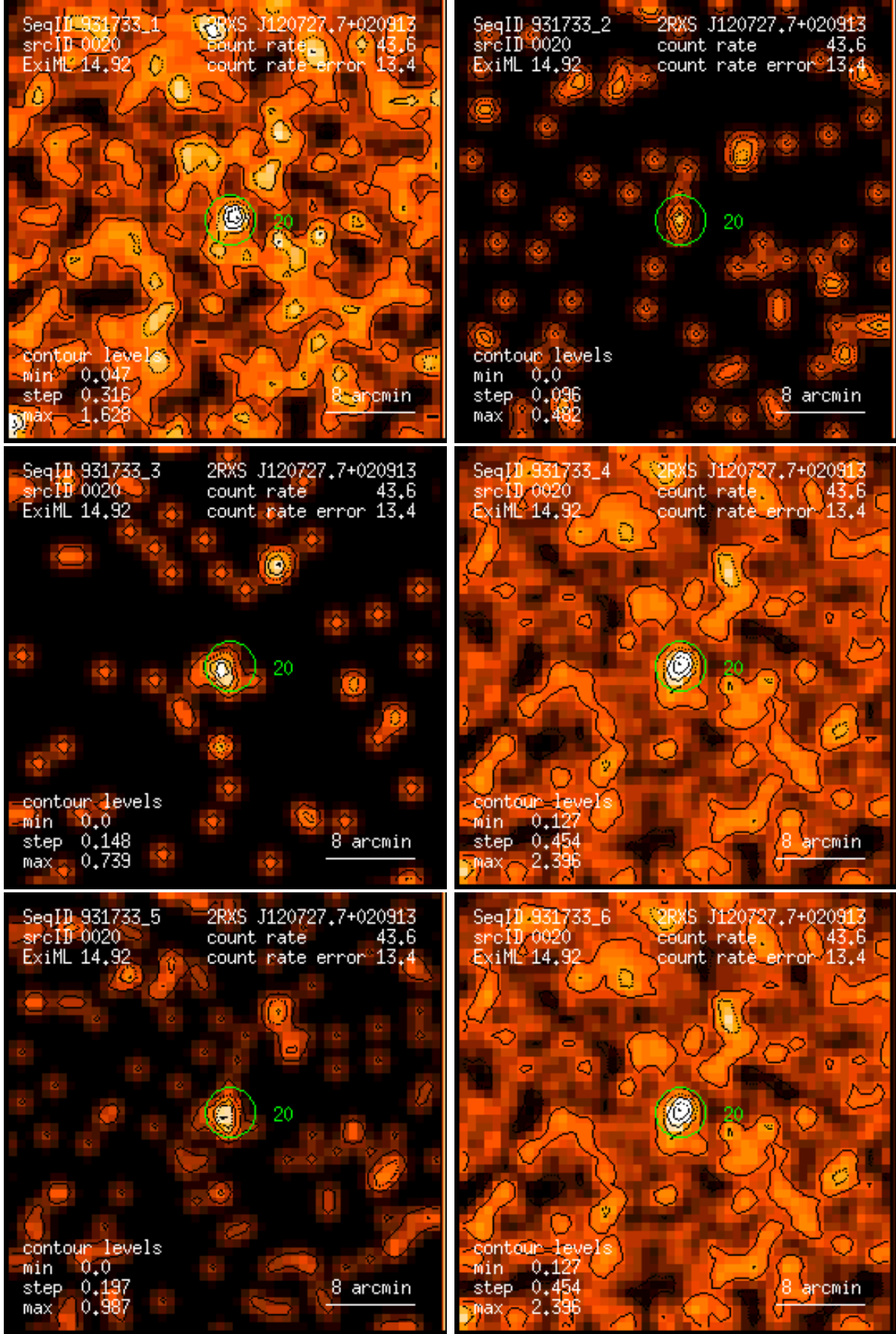
Figure 20: RASS 931733: detection 0020: band rate images, Gaussian filter: (1) PSPC channels 11 – 41, (2) 52 – 90, (3) 91 – 201, (4) 11 – 235, (5) 52 – 201, (6) 11 – 201. Broad band rates in counts/ks. Band rate contour levels in counts/ks/arcmin 2 .
