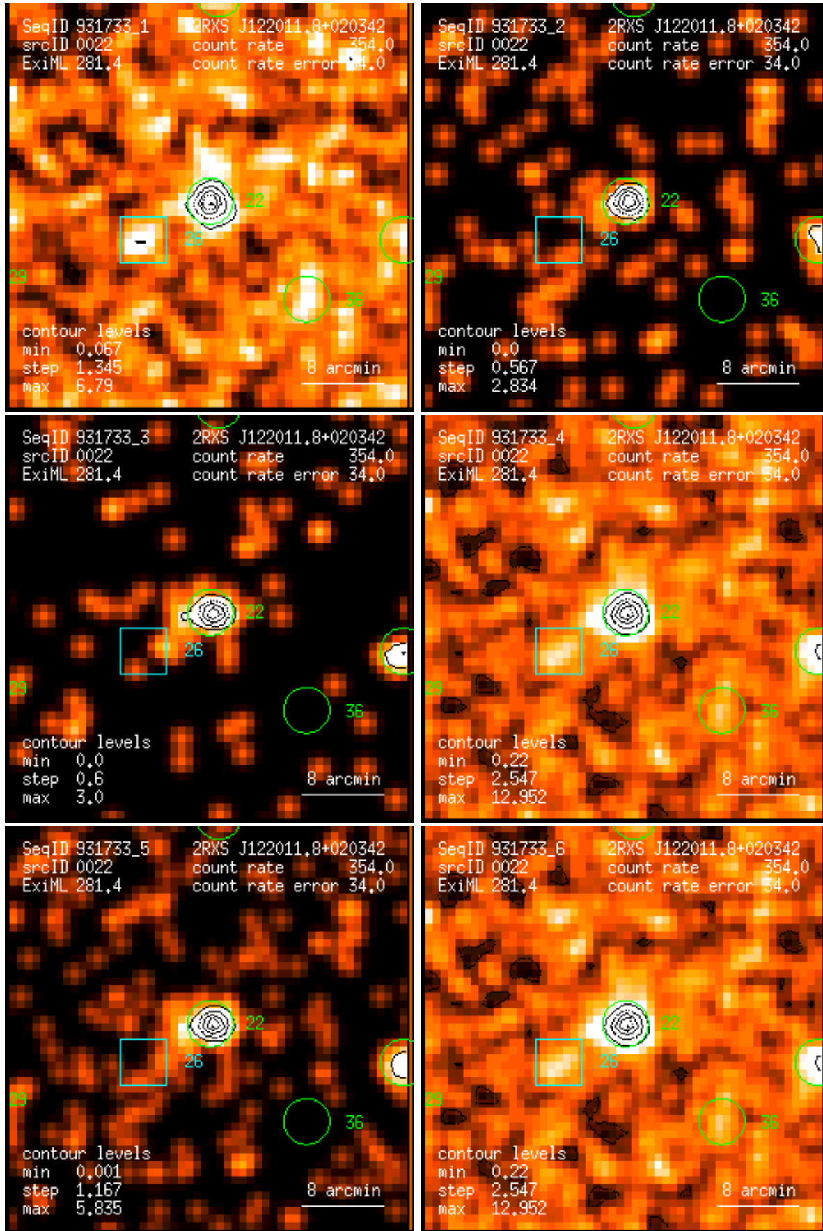
Figure 22: RASS 931733: detection 0022: band rate images, Gaussian filter: (1) PSPC channels 11 – 41, (2) 52 – 90, (3) 91 – 201, (4) 11 – 235, (5) 52 – 201, (6) 11 – 201. Broad band rates in counts/ks. Band rate contour levels in counts/ks/arcmin 2 .
