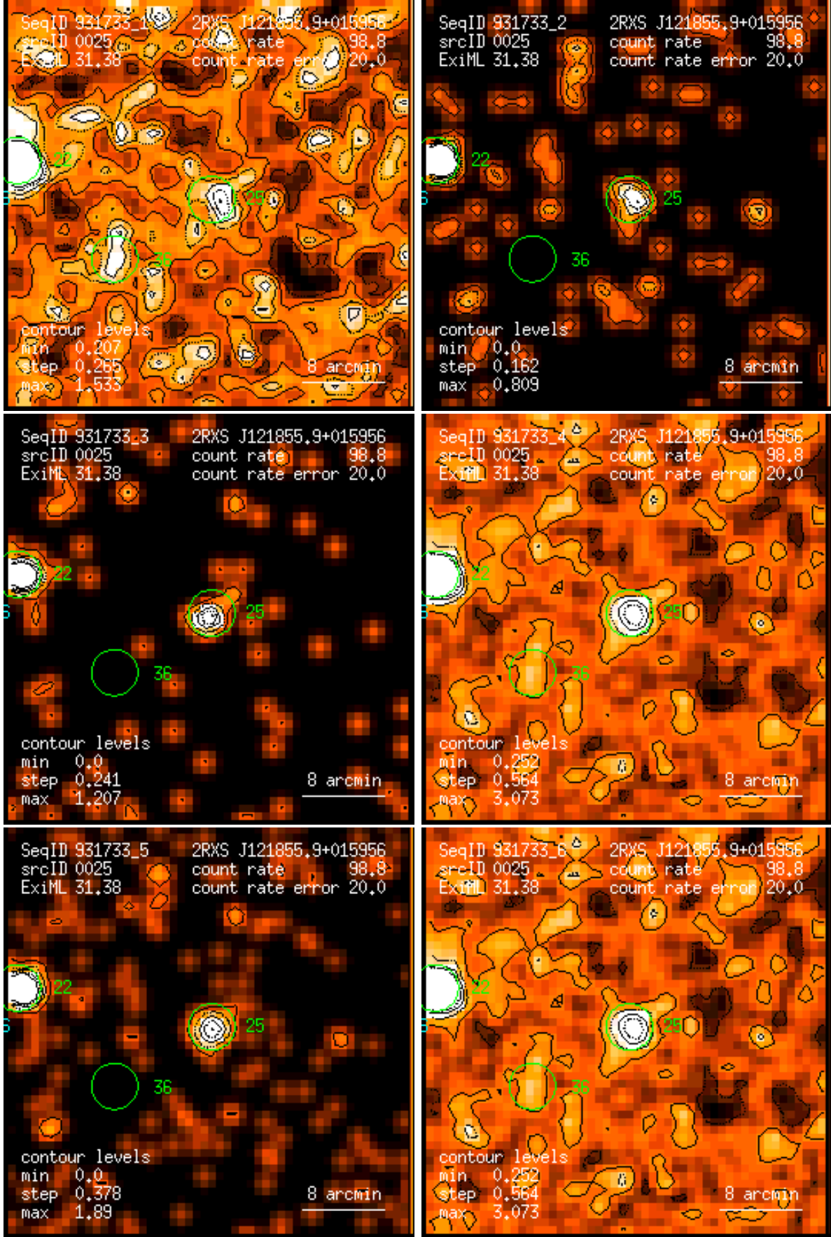
Figure 25: RASS 931733: detection 0025: band rate images, Gaussian filter: (1) PSPC channels 11 – 41, (2) 52 – 90, (3) 91 – 201, (4) 11 – 235, (5) 52 – 201, (6) 11 – 201. Broad band rates in counts/ks. Band rate contour levels in counts/ks/arcmin 2 .
