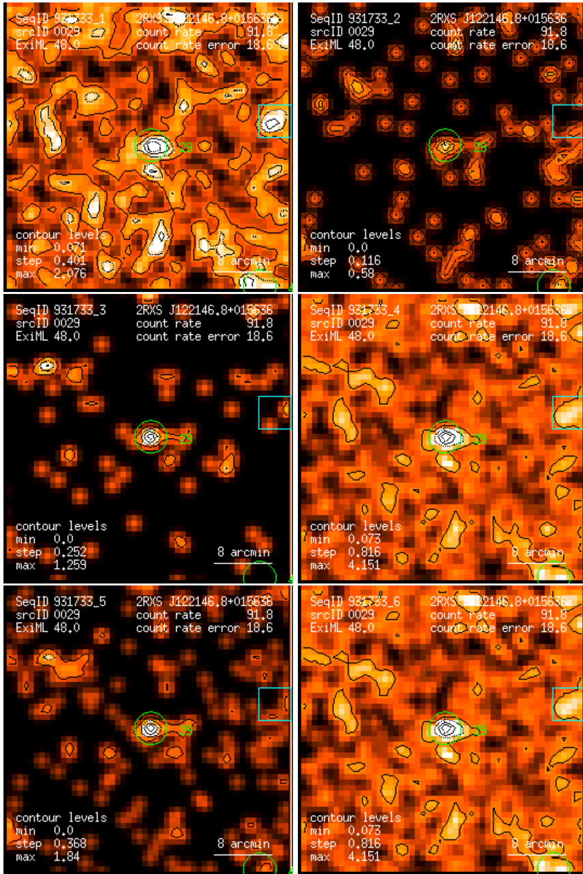
Figure 29: RASS 931733: detection 0029: band rate images, Gaussian filter: (1) PSPC channels 11 – 41, (2) 52 – 90, (3) 91 – 201, (4) 11 – 235, (5) 52 – 201, (6) 11 – 201. Broad band rates in counts/ks. Band rate contour levels in counts/ks/arcmin 2 .
