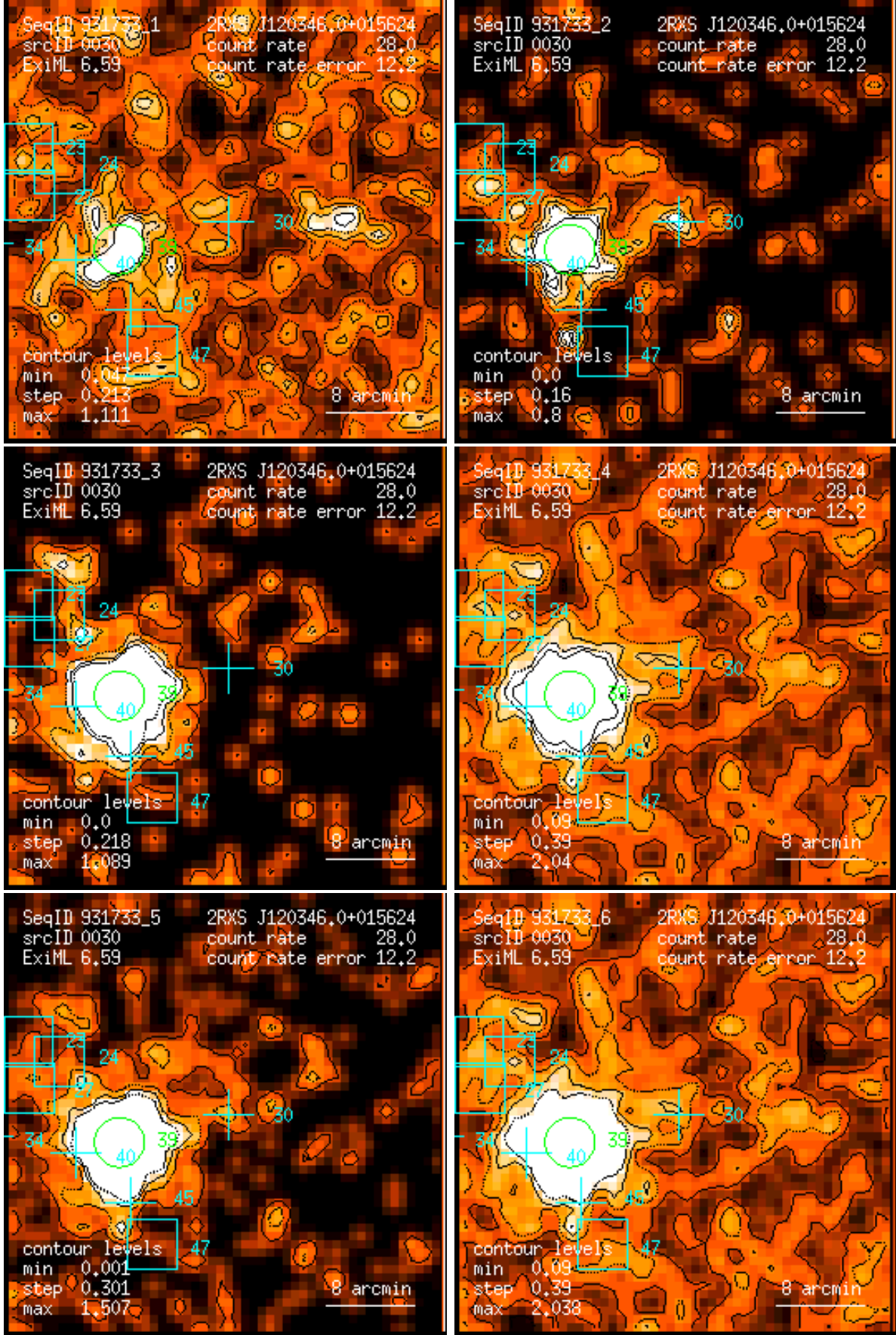
Figure 30: RASS 931733: detection 0030: band rate images, Gaussian filter: (1) PSPC channels 11 – 41, (2) 52 – 90, (3) 91 – 201, (4) 11 – 235, (5) 52 – 201, (6) 11 – 201. Broad band rates in counts/ks. Band rate contour levels in counts/ks/arcmin 2 .
