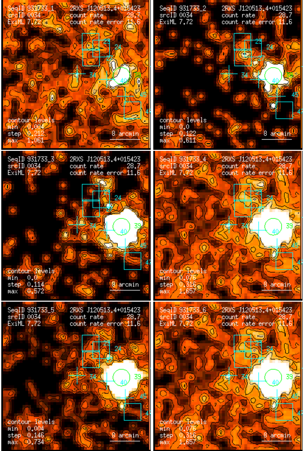
Figure 34: RASS 931733: detection 0034: band rate images, Gaussian filter: (1) PSPC channels 11 – 41, (2) 52 – 90, (3) 91 – 201, (4) 11 – 235, (5) 52 – 201, (6) 11 – 201. Broad band rates in counts/ks. Band rate contour levels in counts/ks/arcmin 2 .
