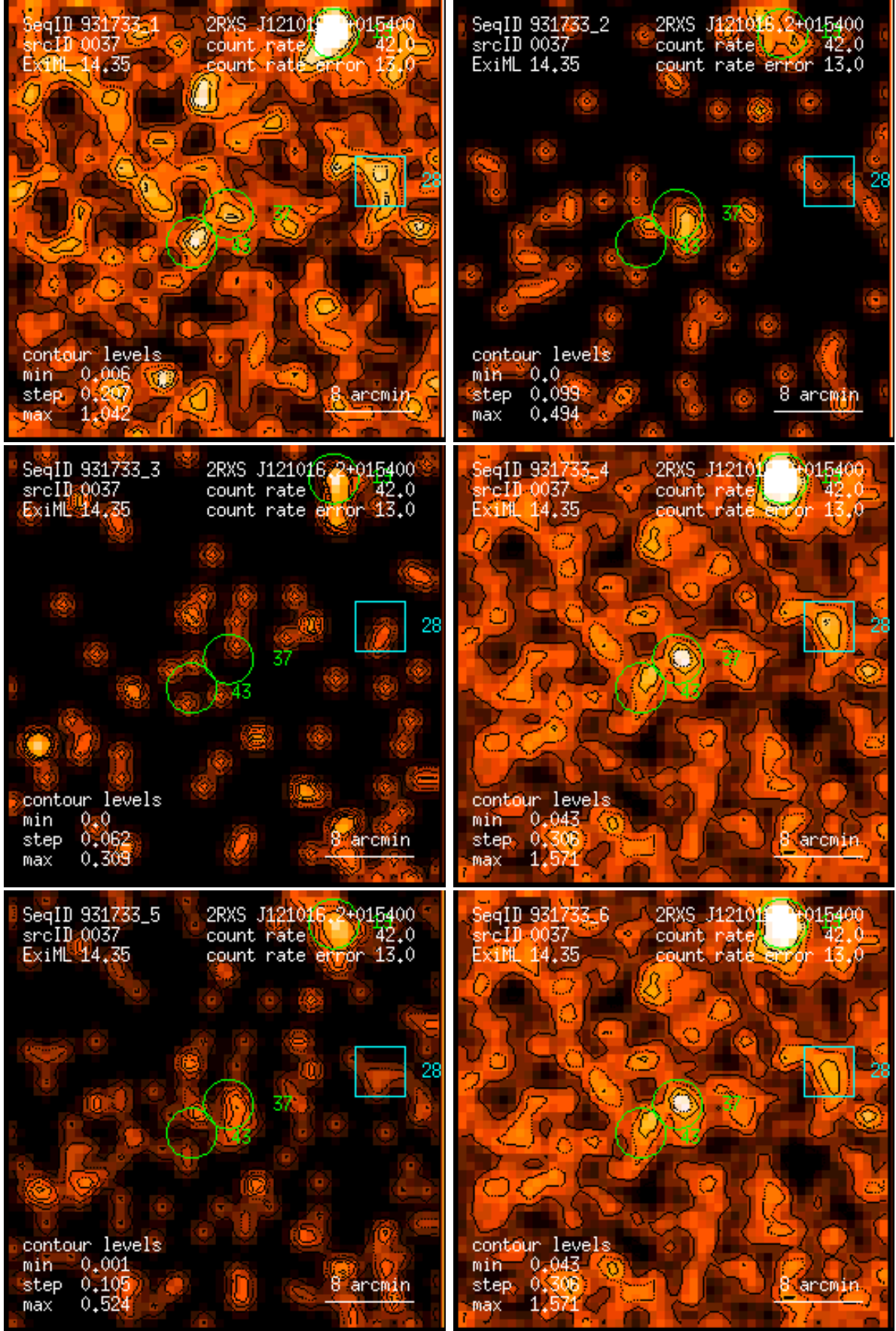
Figure 37: RASS 931733: detection 0037: band rate images, Gaussian filter: (1) PSPC channels 11 – 41, (2) 52 – 90, (3) 91 – 201, (4) 11 – 235, (5) 52 – 201, (6) 11 – 201. Broad band rates in counts/ks. Band rate contour levels in counts/ks/arcmin 2 .
