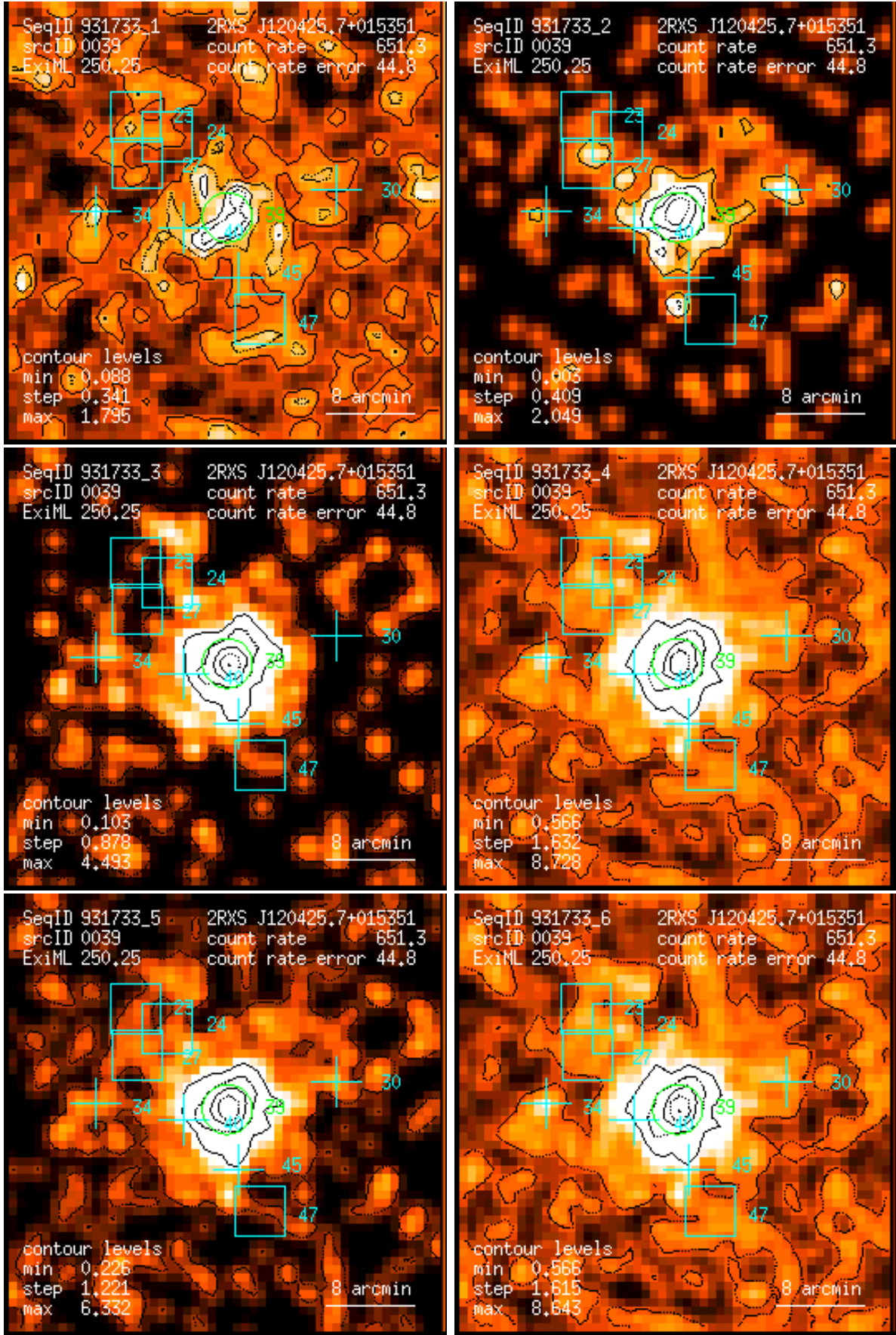
Figure 39: RASS 931733: detection 0039: band rate images, Gaussian filter: (1) PSPC channels 11 – 41, (2) 52 – 90, (3) 91 – 201, (4) 11 – 235, (5) 52 – 201, (6) 11 – 201. Broad band rates in counts/ks. Band rate contour levels in counts/ks/arcmin 2 .
