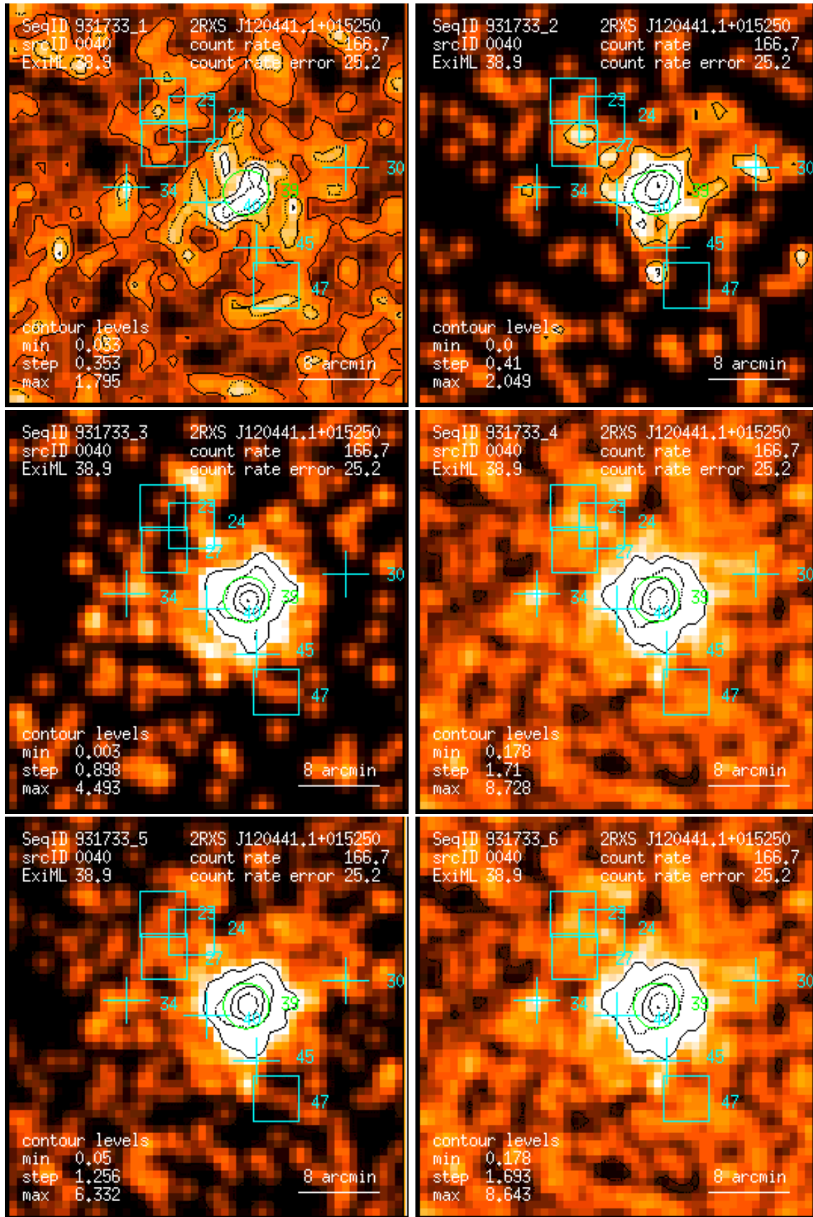
Figure 40: RASS 931733: detection 0040: band rate images, Gaussian filter: (1) PSPC channels 11 – 41, (2) 52 – 90, (3) 91 – 201, (4) 11 – 235, (5) 52 – 201, (6) 11 – 201. Broad band rates in counts/ks. Band rate contour levels in counts/ks/arcmin 2 .
