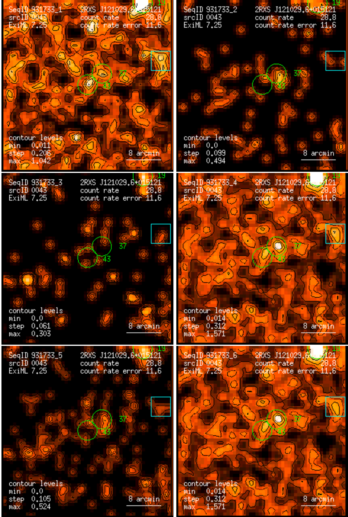
Figure 43: RASS 931733: detection 0043: band rate images, Gaussian filter: (1) PSPC channels 11 – 41, (2) 52 – 90, (3) 91 – 201, (4) 11 – 235, (5) 52 – 201, (6) 11 – 201. Broad band rates in counts/ks. Band rate contour levels in counts/ks/arcmin 2 .
