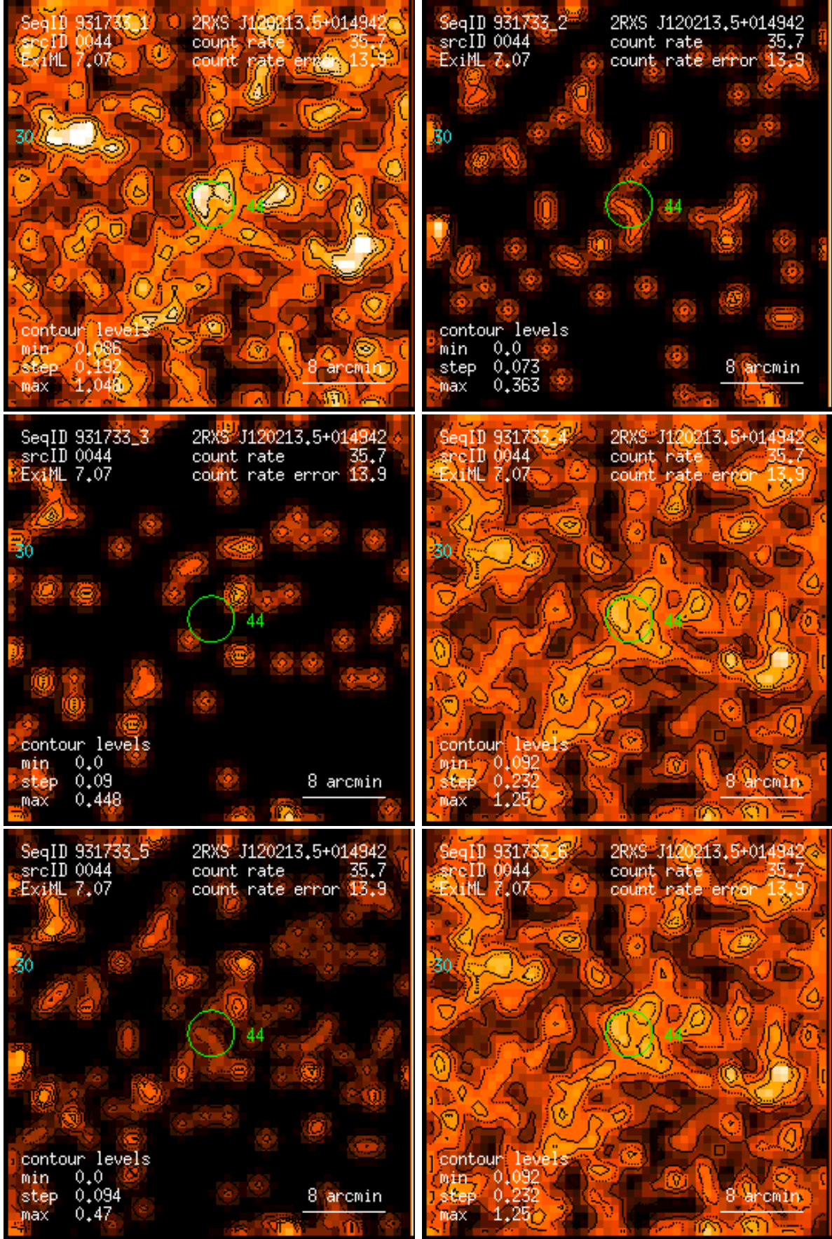
Figure 44: RASS 931733: detection 0044: band rate images, Gaussian filter: (1) PSPC channels 11 – 41, (2) 52 – 90, (3) 91 – 201, (4) 11 – 235, (5) 52 – 201, (6) 11 – 201. Broad band rates in counts/ks. Band rate contour levels in counts/ks/arcmin 2 .
