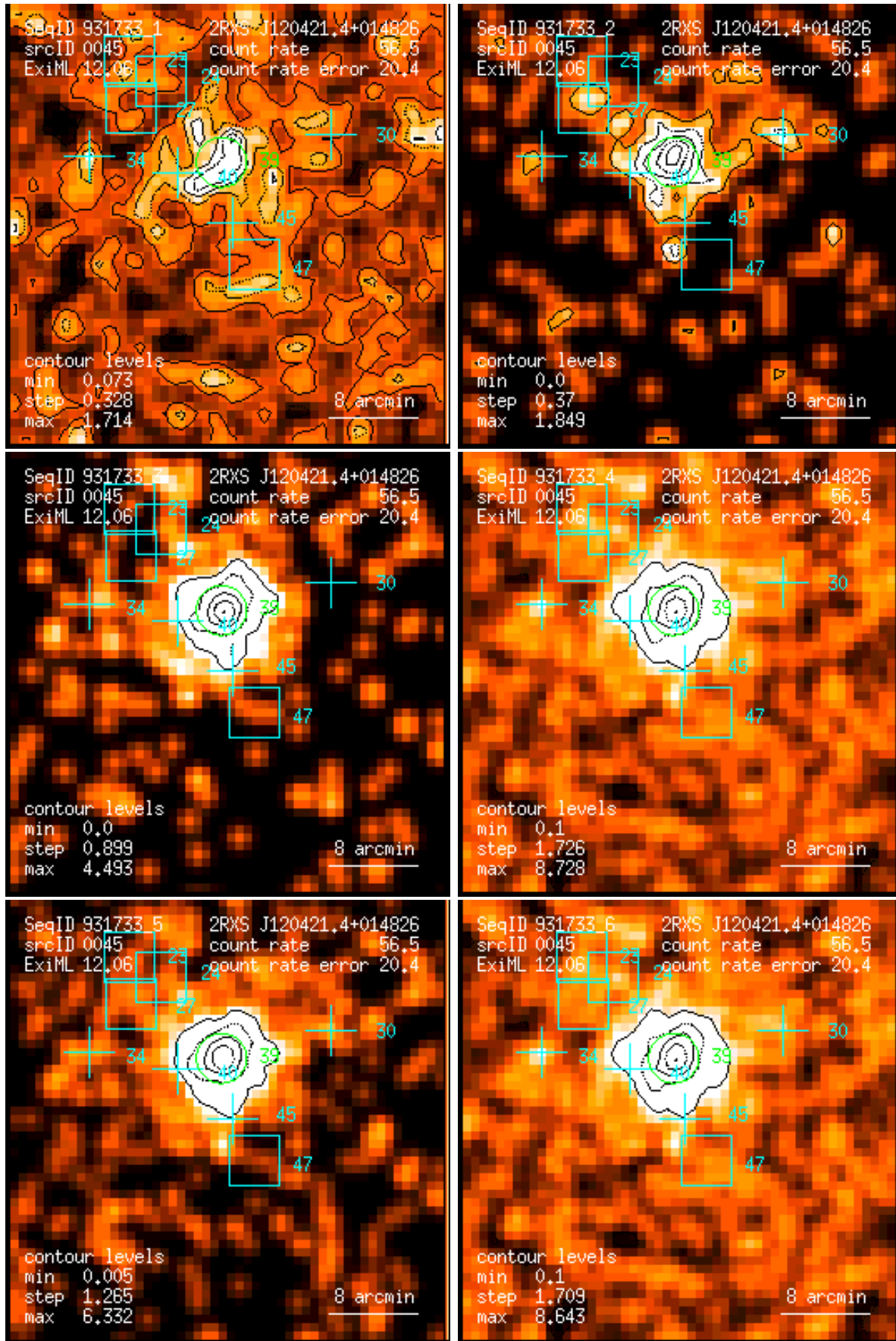
Figure 45: RASS 931733: detection 0045: band rate images, Gaussian filter: (1) PSPC channels 11 – 41, (2) 52 – 90, (3) 91 – 201, (4) 11 – 235, (5) 52 – 201, (6) 11 – 201. Broad band rates in counts/ks. Band rate contour levels in counts/ks/arcmin 2 .
