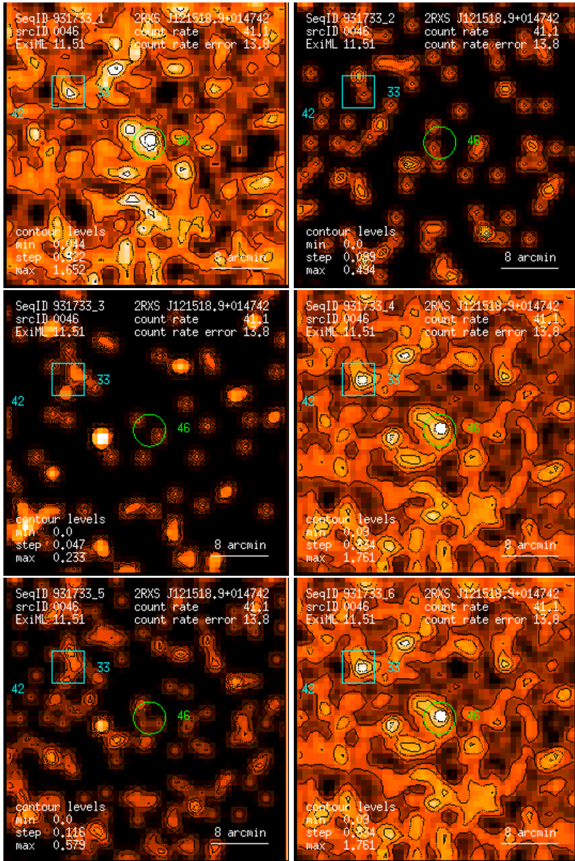
Figure 46: RASS 931733: detection 0046: band rate images, Gaussian filter: (1) PSPC channels 11 – 41, (2) 52 – 90, (3) 91 – 201, (4) 11 – 235, (5) 52 – 201, (6) 11 – 201. Broad band rates in counts/ks. Band rate contour levels in counts/ks/arcmin 2 .
