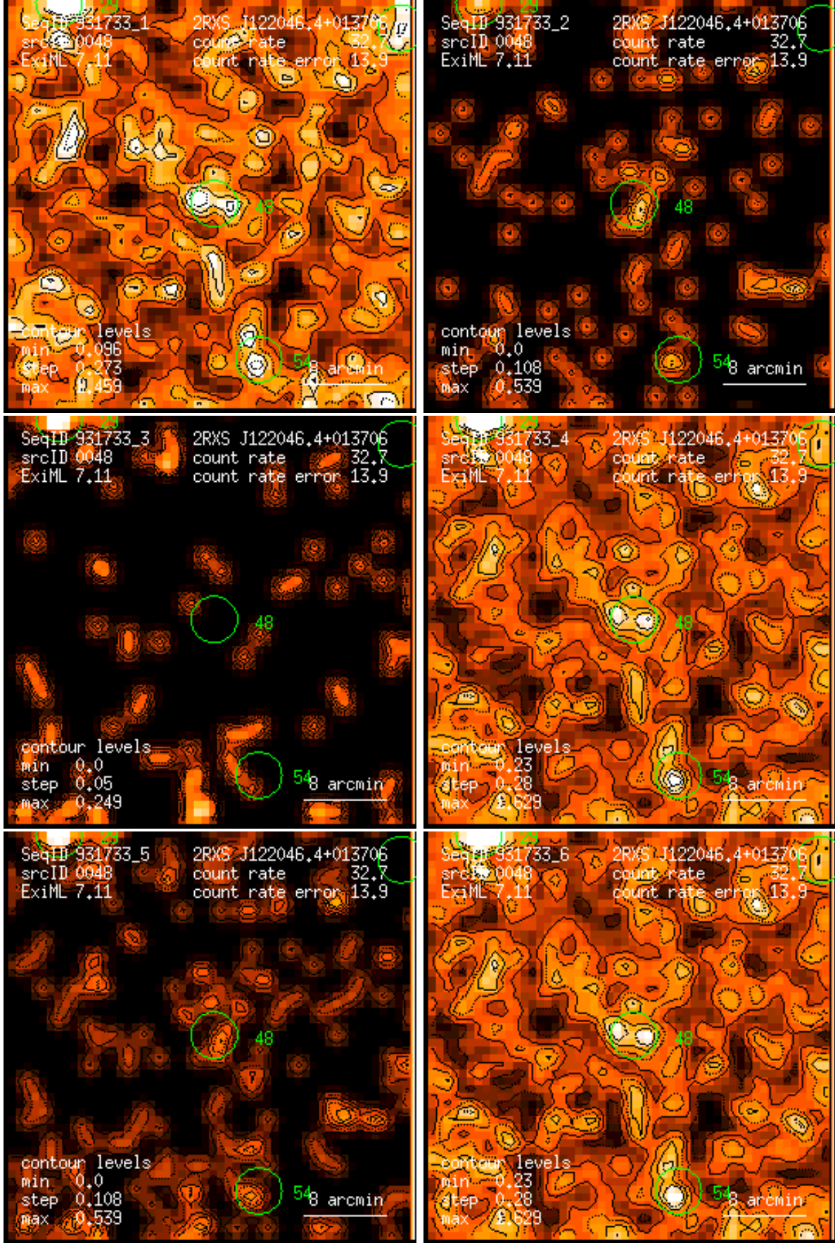
Figure 48: RASS 931733: detection 0048: band rate images, Gaussian filter: (1) PSPC channels 11 – 41, (2) 52 – 90, (3) 91 – 201, (4) 11 – 235, (5) 52 – 201, (6) 11 – 201. Broad band rates in counts/ks. Band rate contour levels in counts/ks/arcmin 2 .
