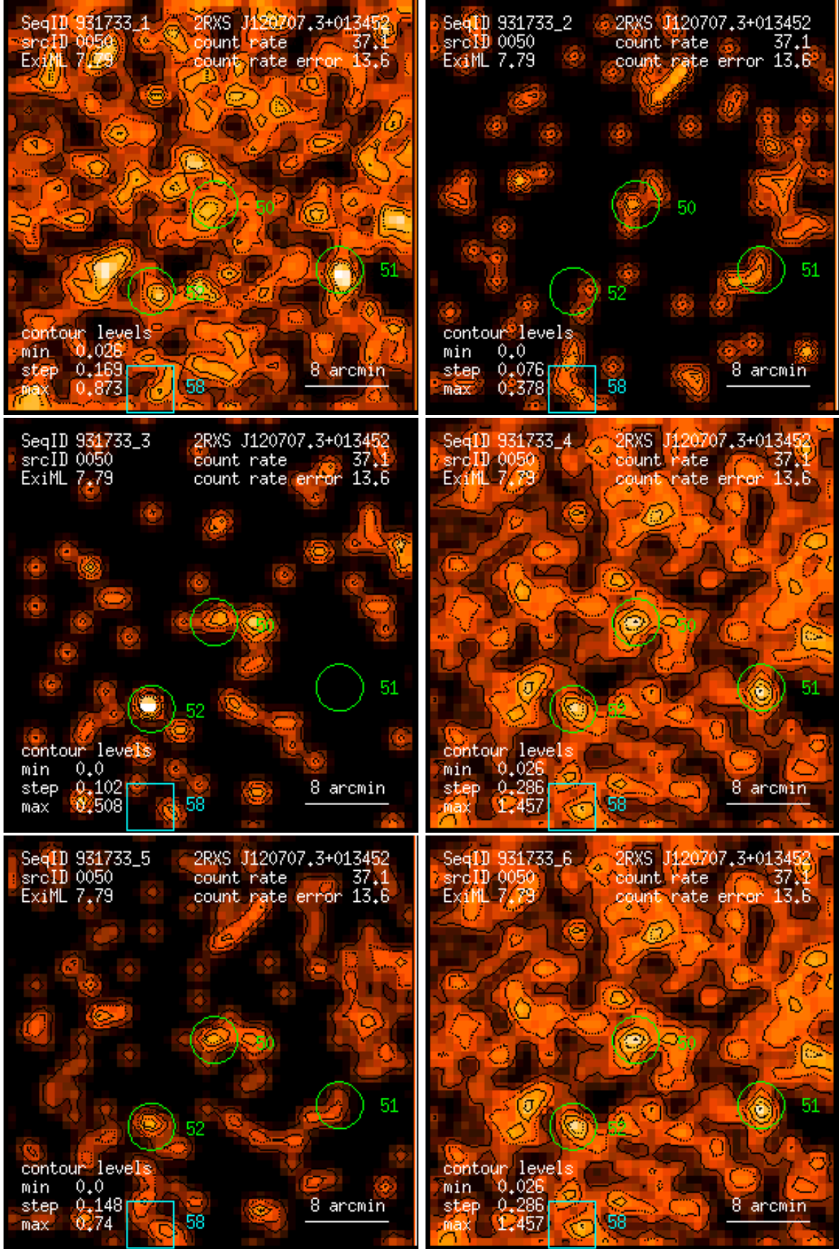
Figure 50: RASS 931733: detection 0050: band rate images, Gaussian filter: (1) PSPC channels 11 – 41, (2) 52 – 90, (3) 91 – 201, (4) 11 – 235, (5) 52 – 201, (6) 11 – 201. Broad band rates in counts/ks. Band rate contour levels in counts/ks/arcmin 2 .
