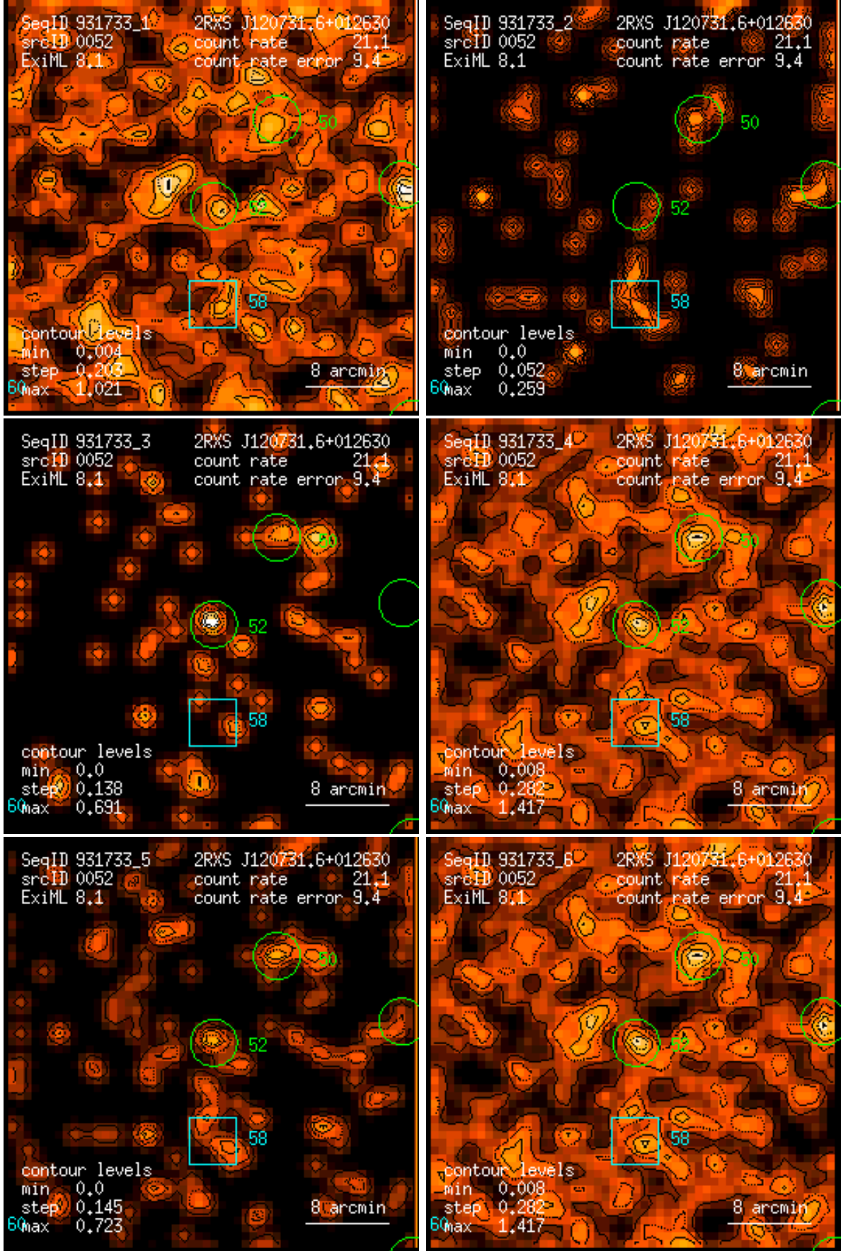
Figure 52: RASS 931733: detection 0052: band rate images, Gaussian filter: (1) PSPC channels 11 – 41, (2) 52 – 90, (3) 91 – 201, (4) 11 – 235, (5) 52 – 201, (6) 11 – 201. Broad band rates in counts/ks. Band rate contour levels in counts/ks/arcmin 2 .
