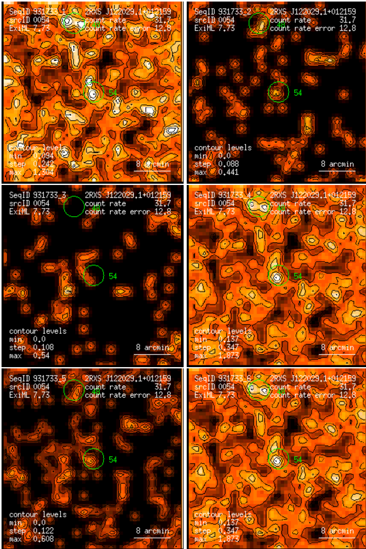
Figure 54: RASS 931733: detection 0054: band rate images, Gaussian filter: (1) PSPC channels 11 – 41, (2) 52 – 90, (3) 91 – 201, (4) 11 – 235, (5) 52 – 201, (6) 11 – 201. Broad band rates in counts/ks. Band rate contour levels in counts/ks/arcmin 2 .
