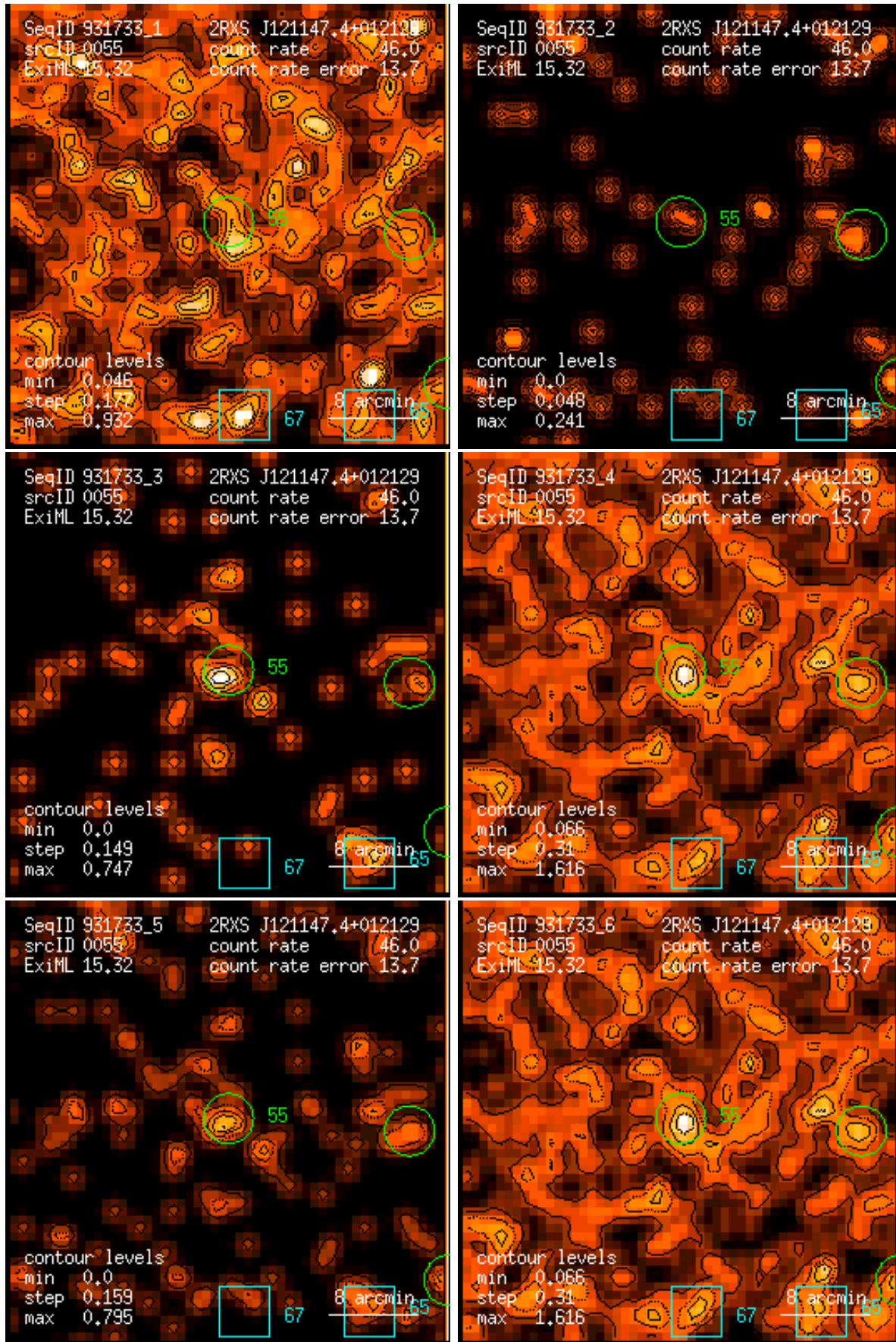
Figure 55: RASS 931733: detection 0055: band rate images, Gaussian filter: (1) PSPC channels 11 – 41, (2) 52 – 90, (3) 91 – 201, (4) 11 – 235, (5) 52 – 201, (6) 11 – 201. Broad band rates in counts/ks. Band rate contour levels in counts/ks/arcmin 2 .
