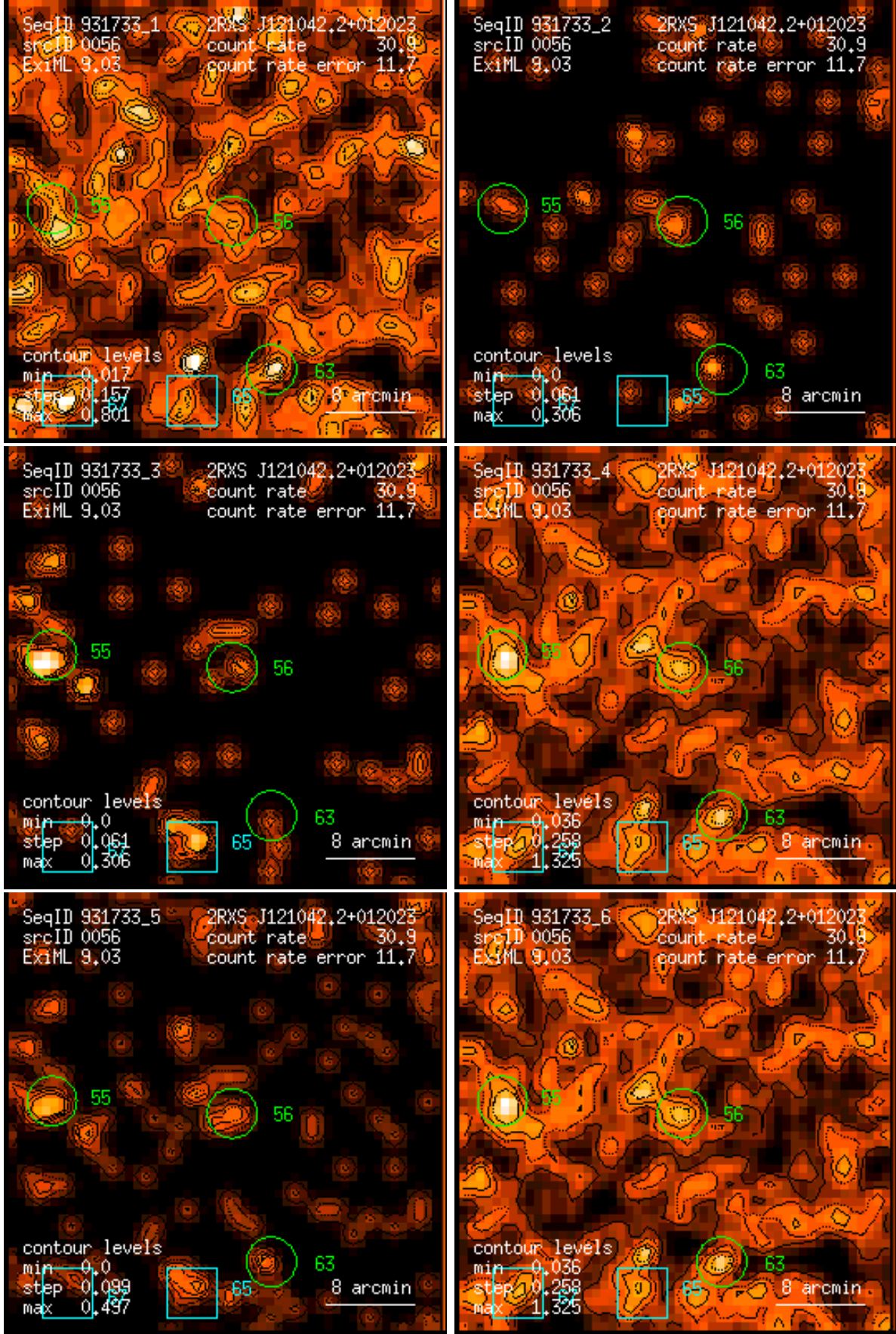
Figure 56: RASS 931733: detection 0056: band rate images, Gaussian filter: (1) PSPC channels 11 – 41, (2) 52 – 90, (3) 91 – 201, (4) 11 – 235, (5) 52 – 201, (6) 11 – 201. Broad band rates in counts/ks. Band rate contour levels in counts/ks/arcmin 2 .
