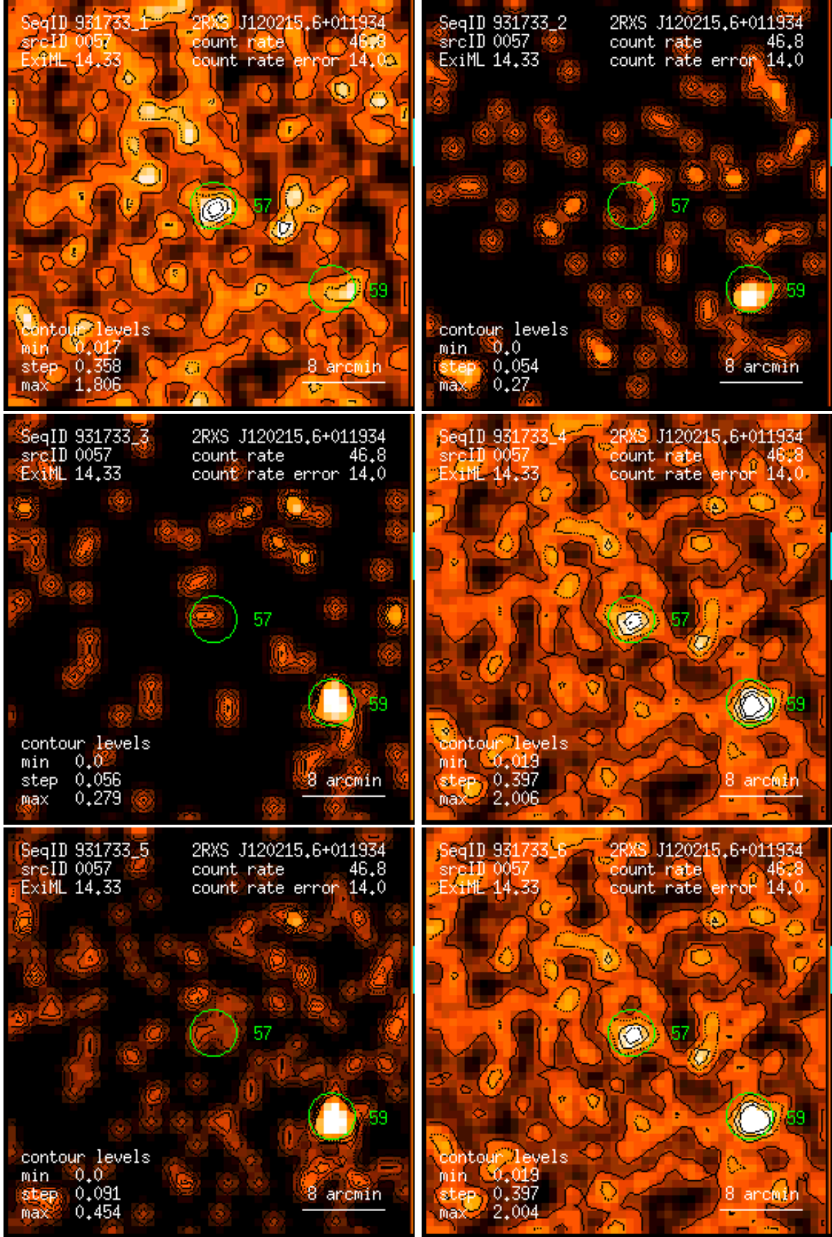
Figure 57: RASS 931733: detection 0057: band rate images, Gaussian filter: (1) PSPC channels 11 – 41, (2) 52 – 90, (3) 91 – 201, (4) 11 – 235, (5) 52 – 201, (6) 11 – 201. Broad band rates in counts/ks. Band rate contour levels in counts/ks/arcmin 2 .
