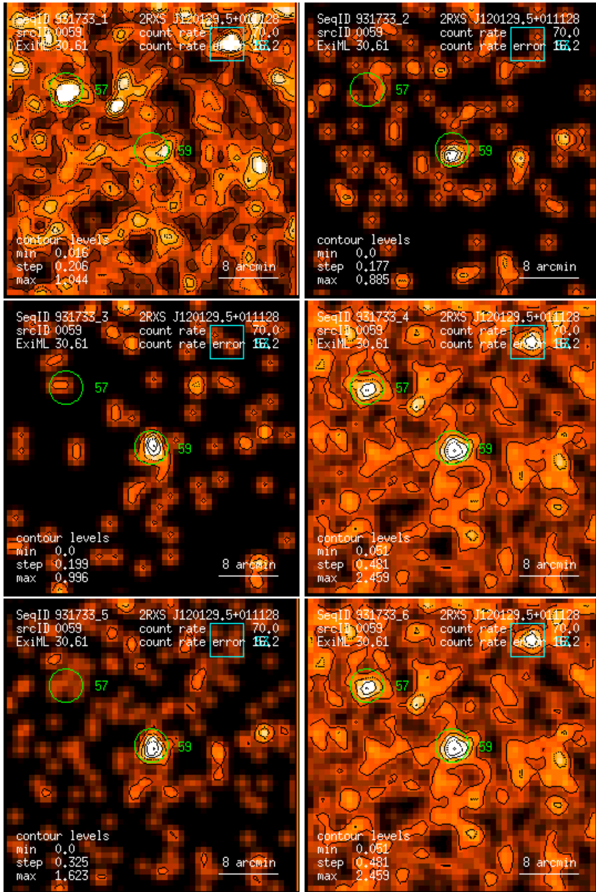
Figure 59: RASS 931733: detection 0059: band rate images, Gaussian filter: (1) PSPC channels 11 – 41, (2) 52 – 90, (3) 91 – 201, (4) 11 – 235, (5) 52 – 201, (6) 11 – 201. Broad band rates in counts/ks. Band rate contour levels in counts/ks/arcmin 2 .
