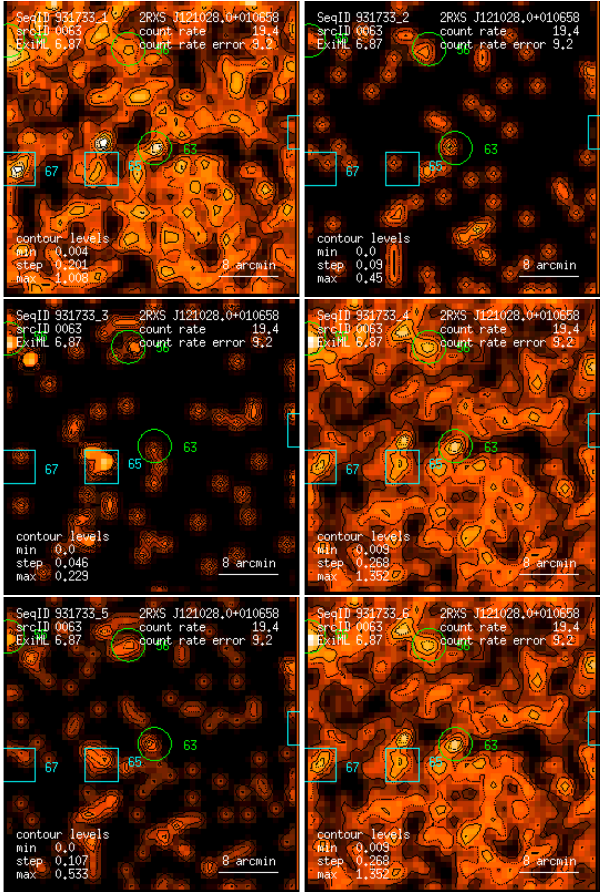
Figure 63: RASS 931733: detection 0063: band rate images, Gaussian filter: (1) PSPC channels 11 – 41, (2) 52 – 90, (3) 91 – 201, (4) 11 – 235, (5) 52 – 201, (6) 11 – 201. Broad band rates in counts/ks. Band rate contour levels in counts/ks/arcmin 2 .
