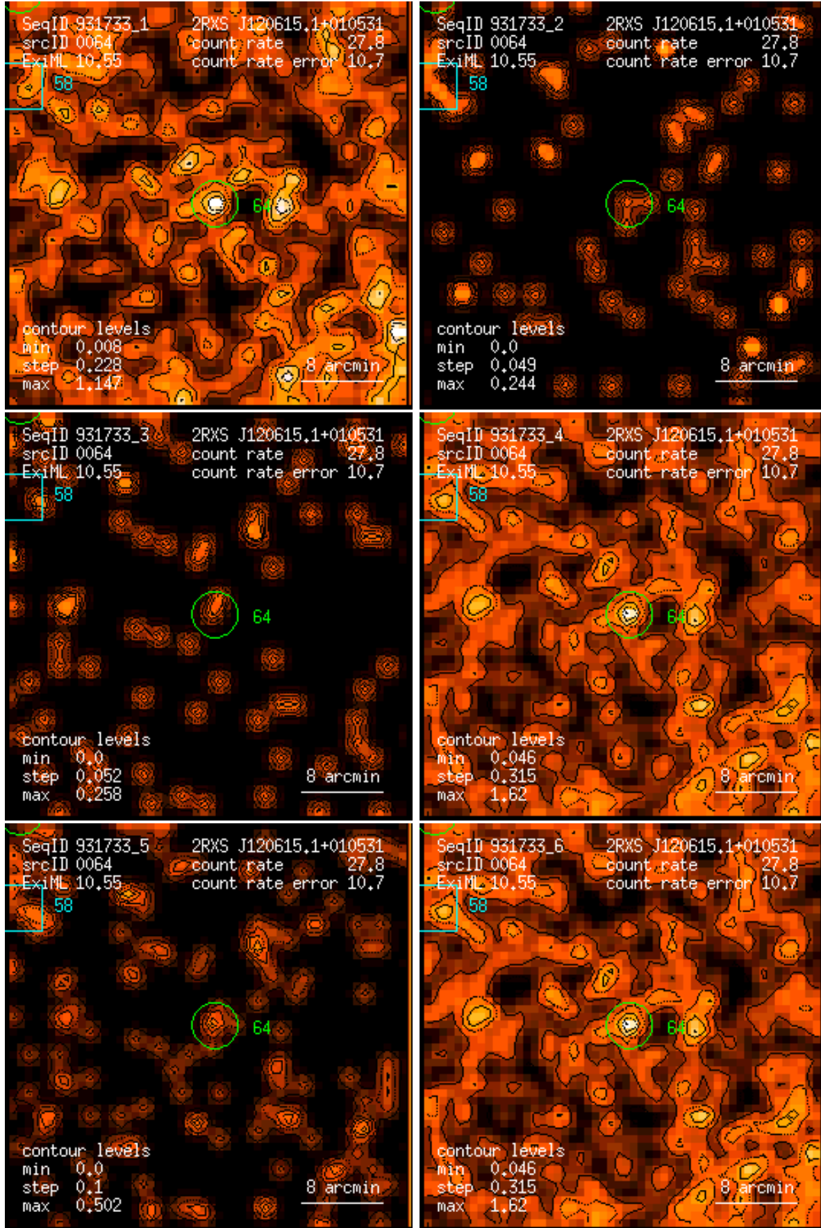
Figure 64: RASS 931733: detection 0064: band rate images, Gaussian filter: (1) PSPC channels 11 – 41, (2) 52 – 90, (3) 91 – 201, (4) 11 – 235, (5) 52 – 201, (6) 11 – 201. Broad band rates in counts/ks. Band rate contour levels in counts/ks/arcmin 2 .
