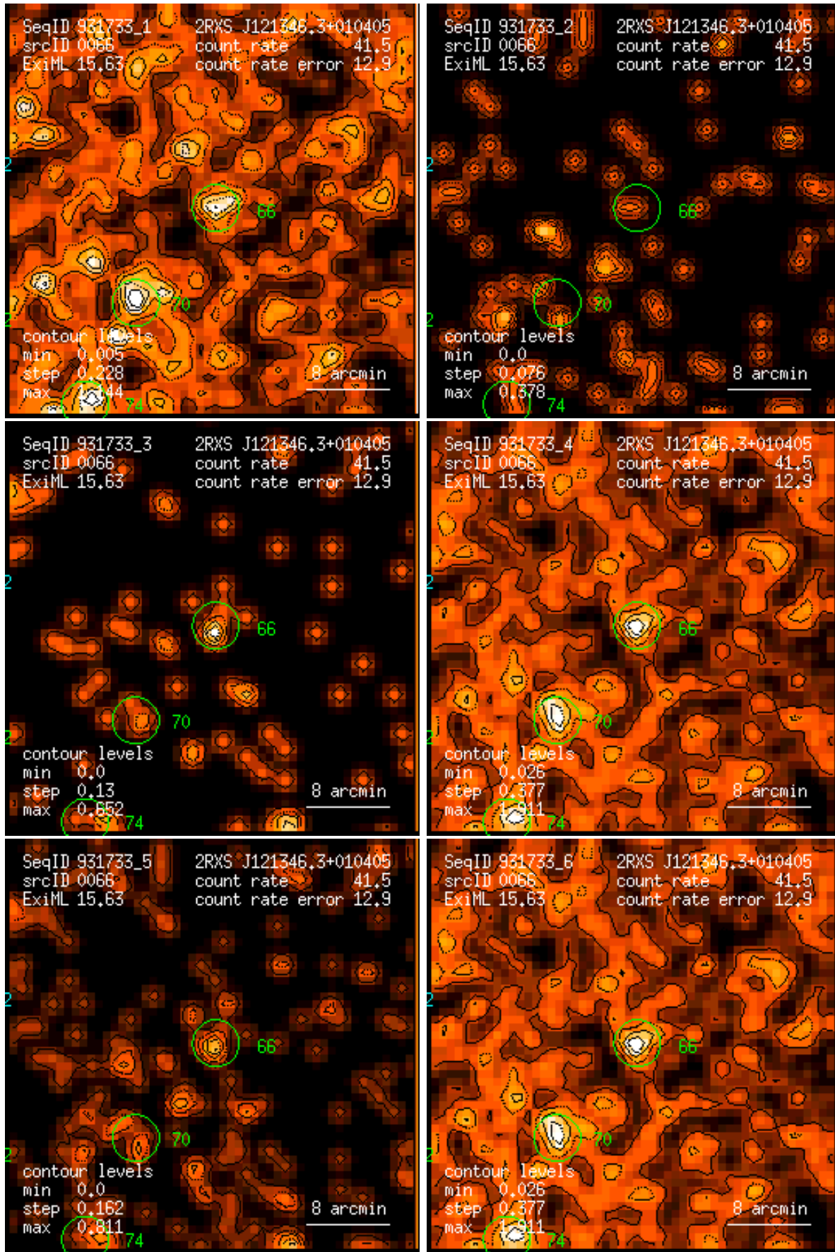
Figure 66: RASS 931733: detection 0066: band rate images, Gaussian filter: (1) PSPC channels 11 – 41, (2) 52 – 90, (3) 91 – 201, (4) 11 – 235, (5) 52 – 201, (6) 11 – 201. Broad band rates in counts/ks. Band rate contour levels in counts/ks/arcmin 2 .
