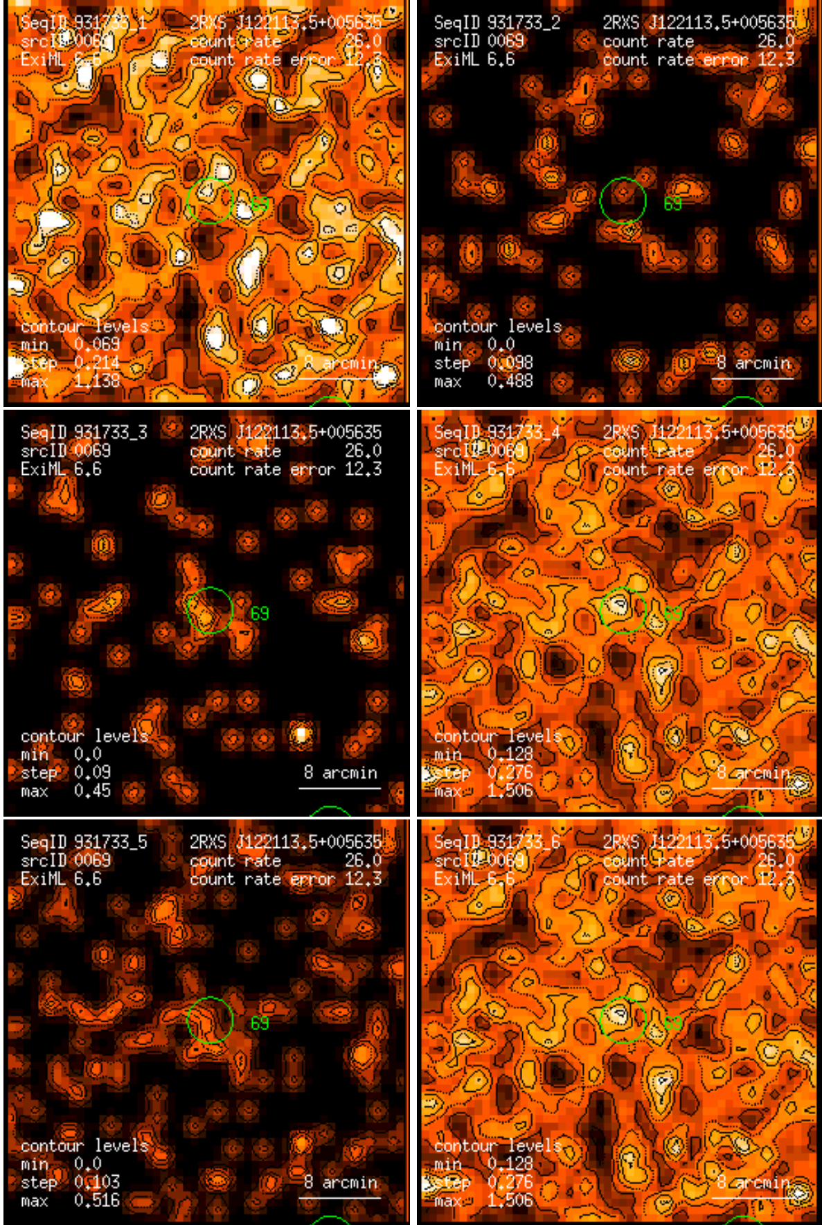
Figure 69: RASS 931733: detection 0069: band rate images, Gaussian filter: (1) PSPC channels 11 – 41, (2) 52 – 90, (3) 91 – 201, (4) 11 – 235, (5) 52 – 201, (6) 11 – 201. Broad band rates in counts/ks. Band rate contour levels in counts/ks/arcmin 2 .
