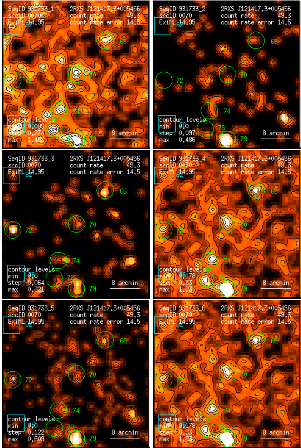
Figure 70: RASS 931733: detection 0070: band rate images, Gaussian filter: (1) PSPC channels 11 – 41, (2) 52 – 90, (3) 91 – 201, (4) 11 – 235, (5) 52 – 201, (6) 11 – 201. Broad band rates in counts/ks. Band rate contour levels in counts/ks/arcmin 2 .
