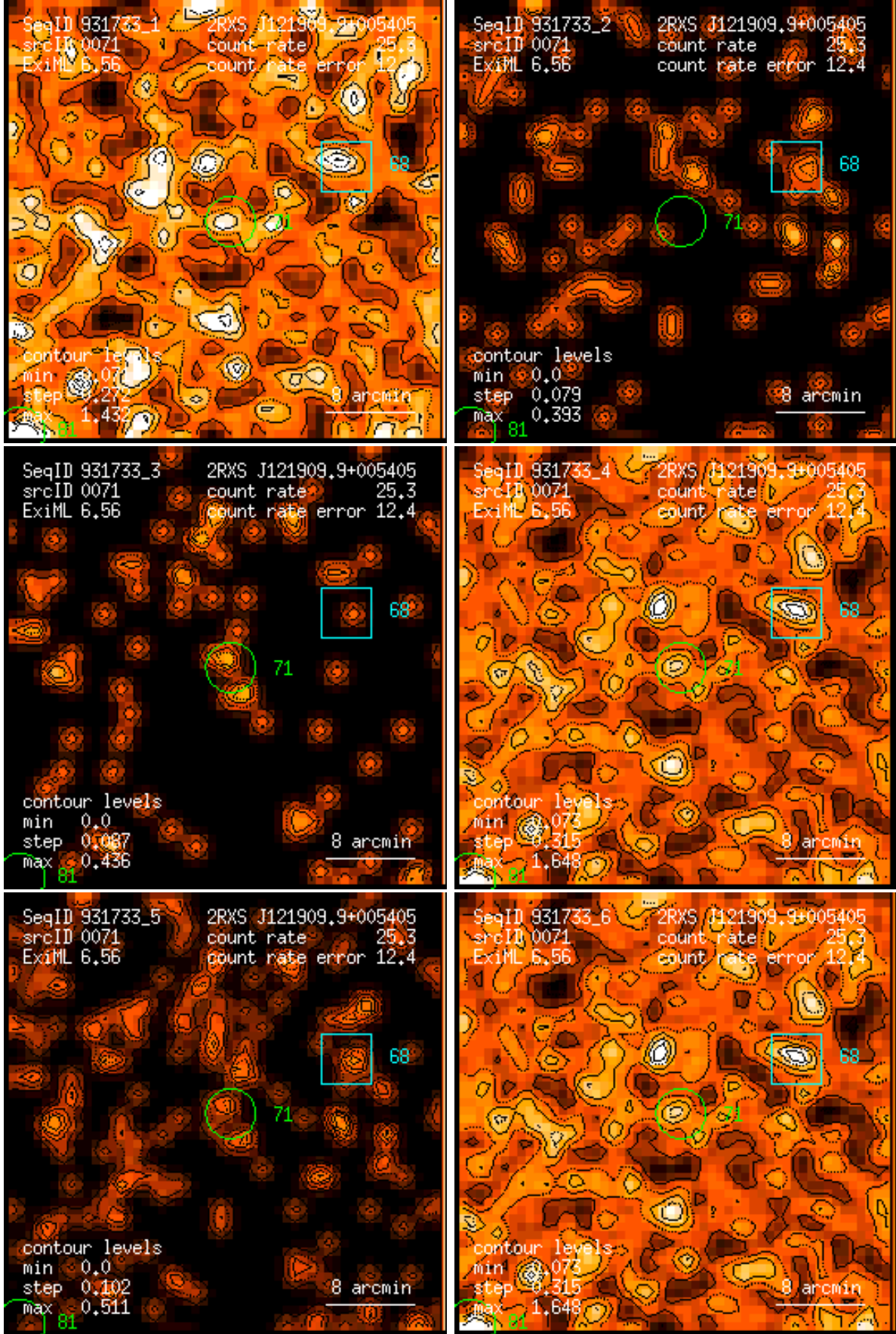
Figure 71: RASS 931733: detection 0071: band rate images, Gaussian filter: (1) PSPC channels 11 – 41, (2) 52 – 90, (3) 91 – 201, (4) 11 – 235, (5) 52 – 201, (6) 11 – 201. Broad band rates in counts/ks. Band rate contour levels in counts/ks/arcmin 2 .
