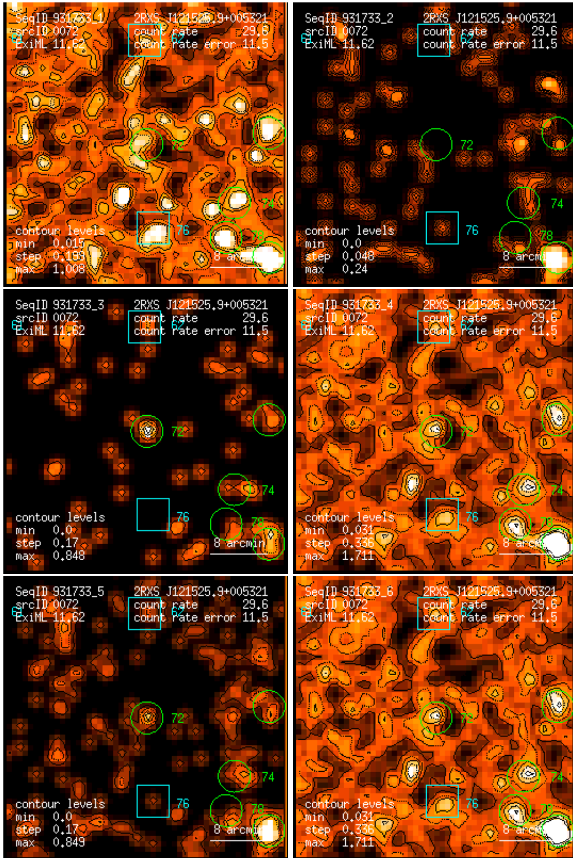
Figure 72: RASS 931733: detection 0072: band rate images, Gaussian filter: (1) PSPC channels 11 – 41, (2) 52 – 90, (3) 91 – 201, (4) 11 – 235, (5) 52 – 201, (6) 11 – 201. Broad band rates in counts/ks. Band rate contour levels in counts/ks/arcmin 2 .
