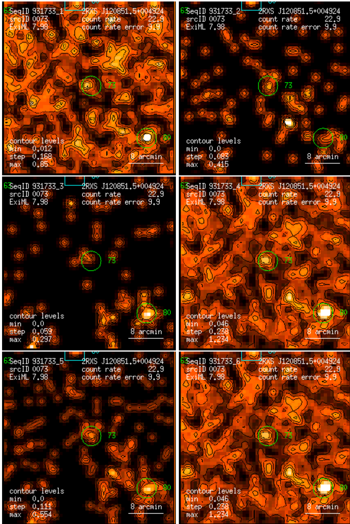
Figure 73: RASS 931733: detection 0073: band rate images, Gaussian filter: (1) PSPC channels 11 – 41, (2) 52 – 90, (3) 91 – 201, (4) 11 – 235, (5) 52 – 201, (6) 11 – 201. Broad band rates in counts/ks. Band rate contour levels in counts/ks/arcmin 2 .
