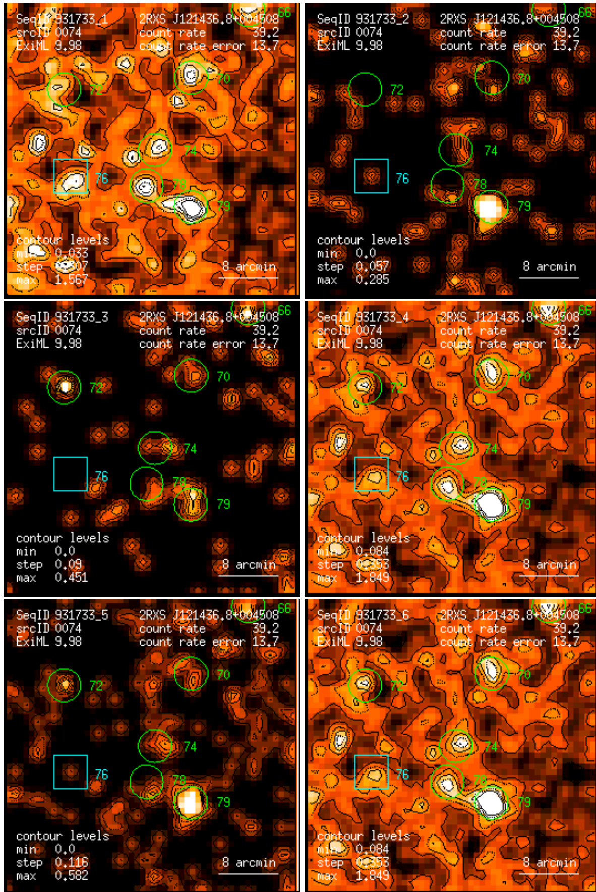
Figure 74: RASS 931733: detection 0074: band rate images, Gaussian filter: (1) PSPC channels 11 – 41, (2) 52 – 90, (3) 91 – 201, (4) 11 – 235, (5) 52 – 201, (6) 11 – 201. Broad band rates in counts/ks. Band rate contour levels in counts/ks/arcmin 2 .
