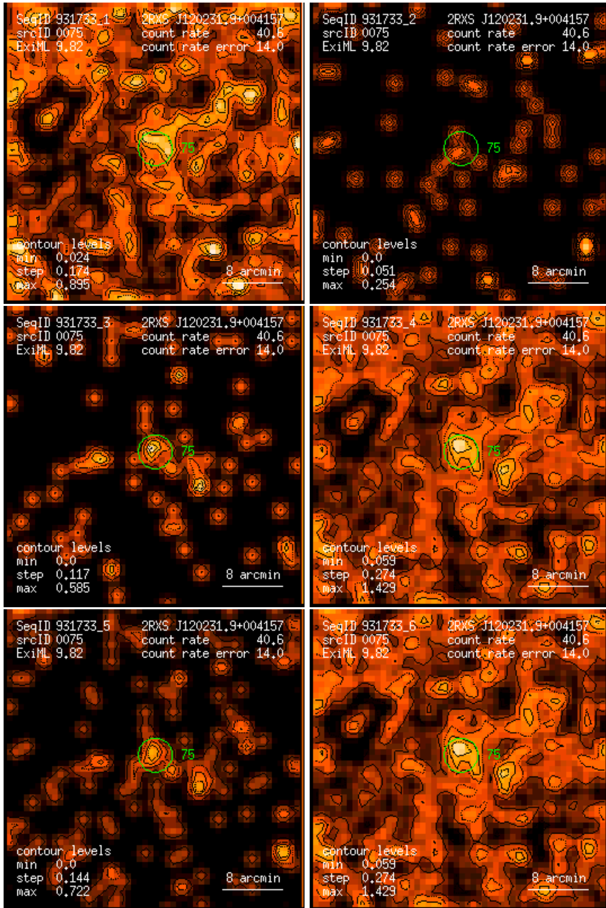
Figure 75: RASS 931733: detection 0075: band rate images, Gaussian filter: (1) PSPC channels 11 – 41, (2) 52 – 90, (3) 91 – 201, (4) 11 – 235, (5) 52 – 201, (6) 11 – 201. Broad band rates in counts/ks. Band rate contour levels in counts/ks/arcmin 2 .
