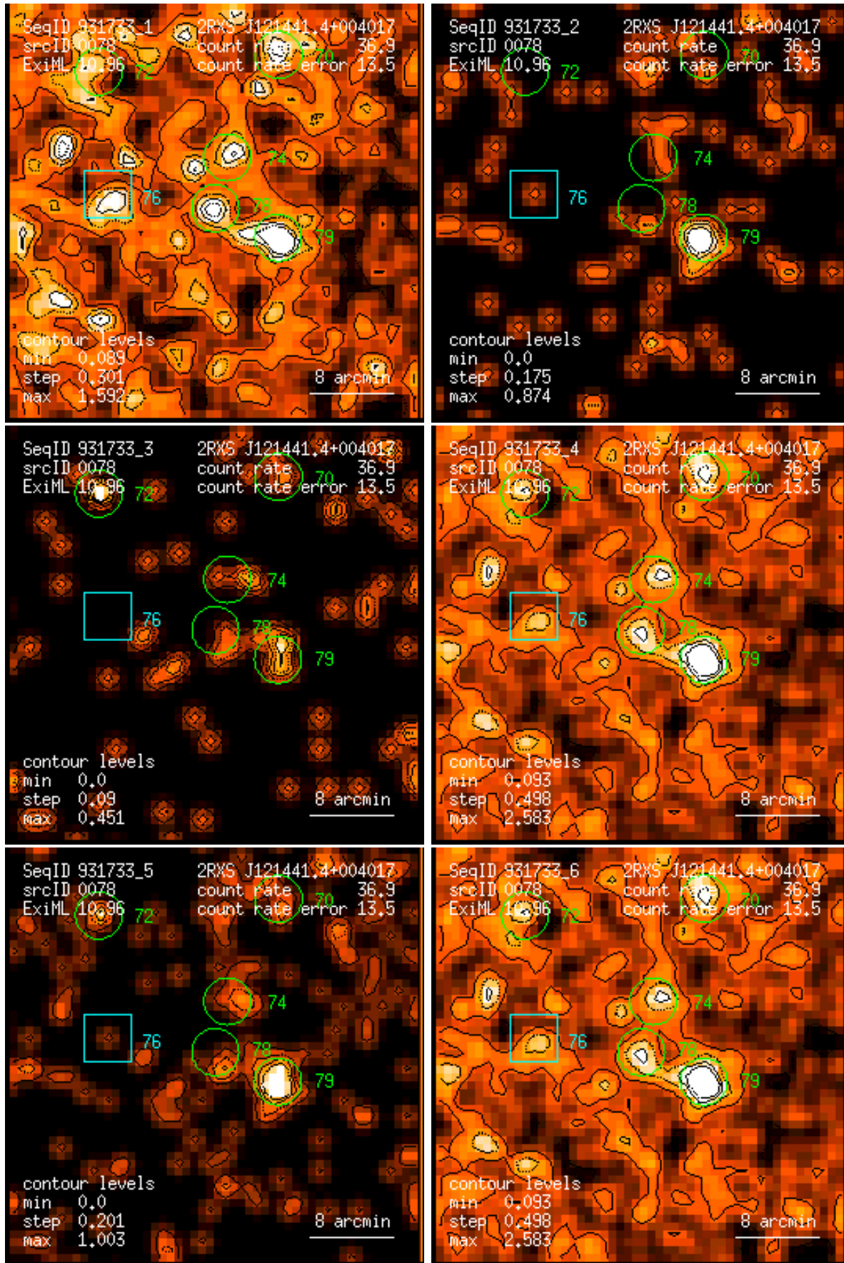
Figure 78: RASS 931733: detection 0078: band rate images, Gaussian filter: (1) PSPC channels 11 – 41, (2) 52 – 90, (3) 91 – 201, (4) 11 – 235, (5) 52 – 201, (6) 11 – 201. Broad band rates in counts/ks. Band rate contour levels in counts/ks/arcmin 2 .
