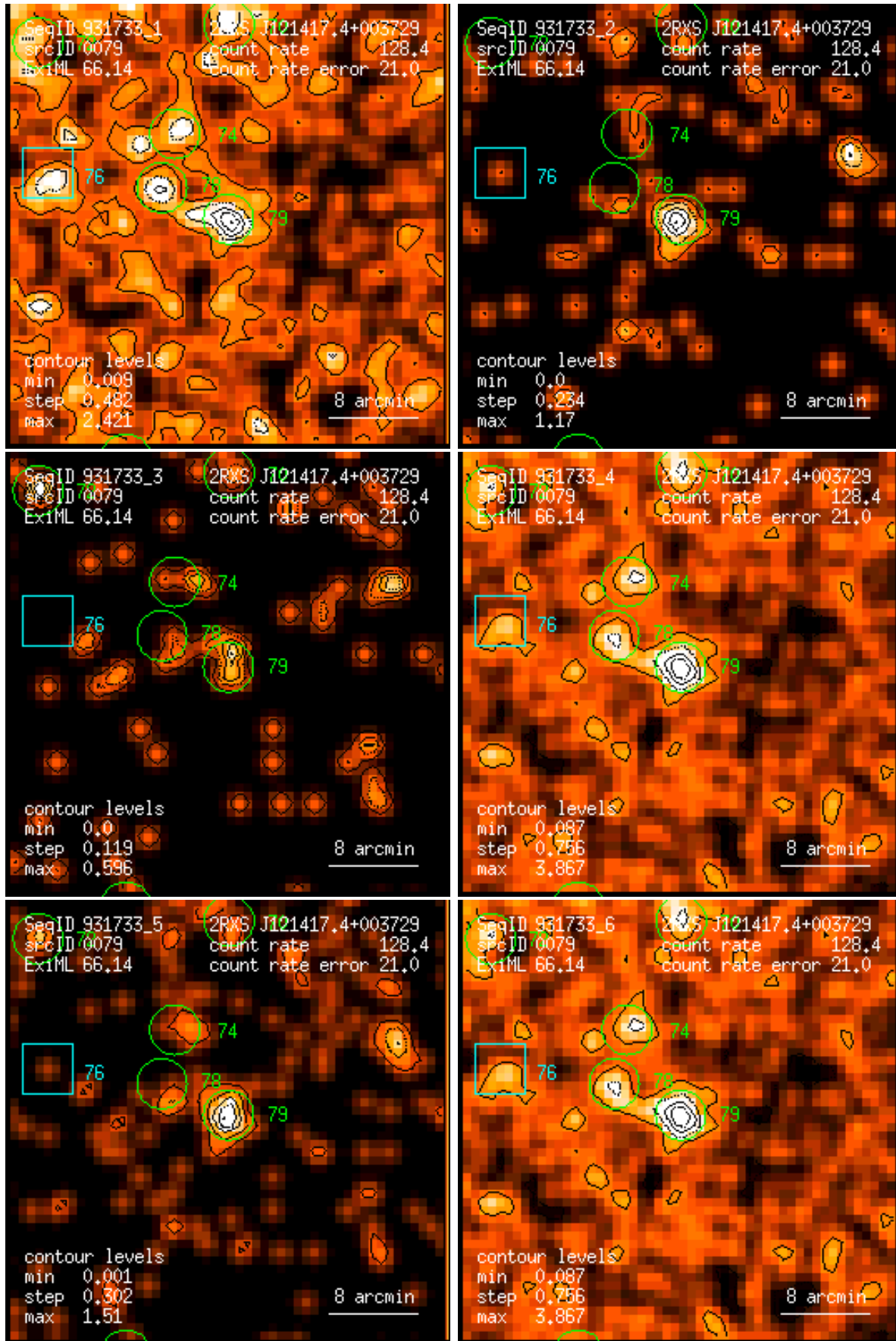
Figure 79: RASS 931733: detection 0079: band rate images, Gaussian filter: (1) PSPC channels 11 – 41, (2) 52 – 90, (3) 91 – 201, (4) 11 – 235, (5) 52 – 201, (6) 11 – 201. Broad band rates in counts/ks. Band rate contour levels in counts/ks/arcmin 2 .
