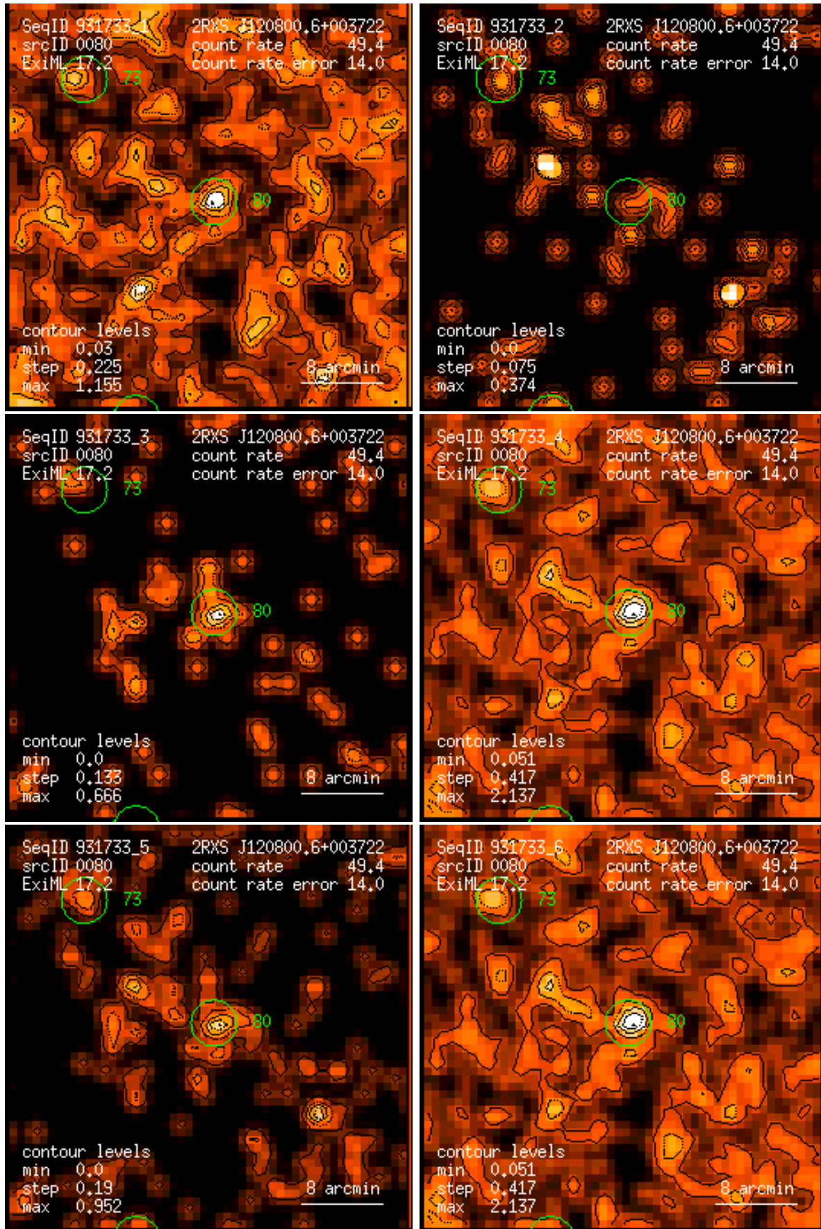
Figure 80: RASS 931733: detection 0080: band rate images, Gaussian filter: (1) PSPC channels 11 – 41, (2) 52 – 90, (3) 91 – 201, (4) 11 – 235, (5) 52 – 201, (6) 11 – 201. Broad band rates in counts/ks. Band rate contour levels in counts/ks/arcmin 2 .
