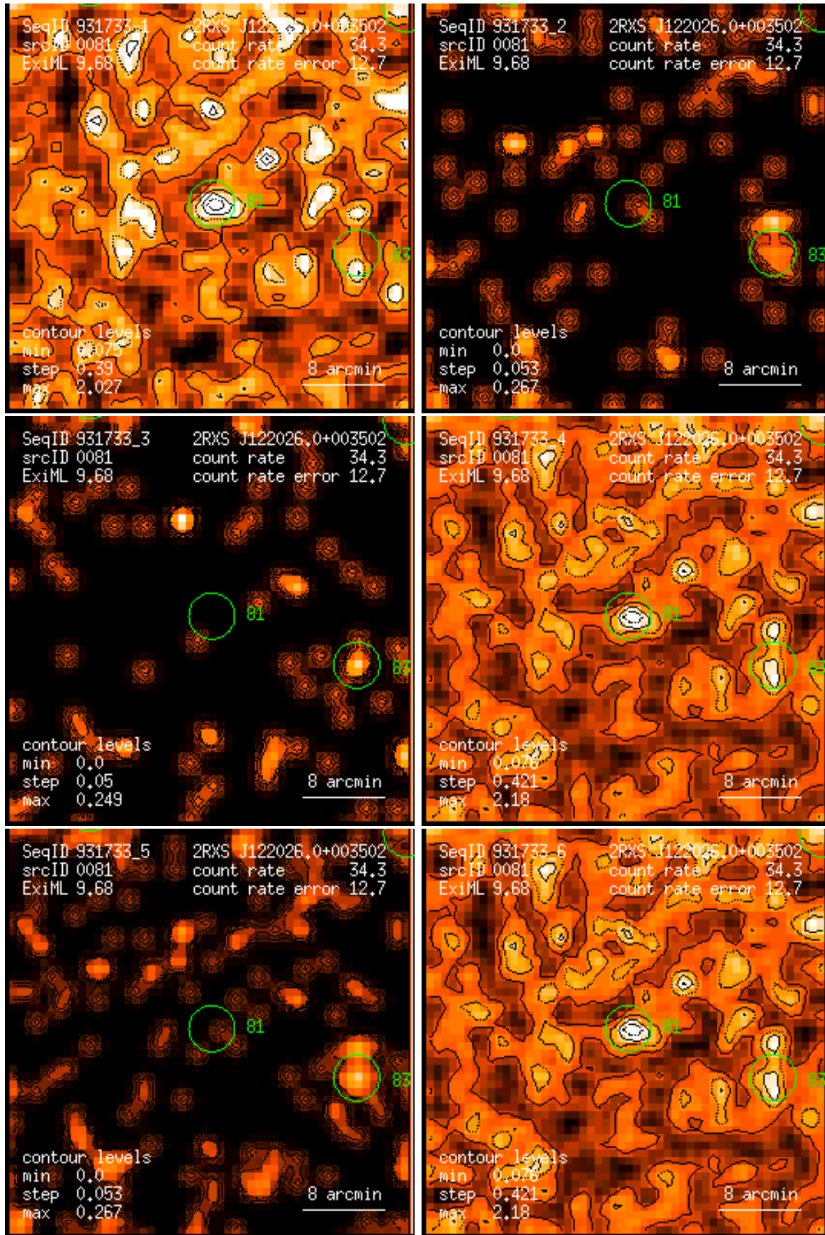
Figure 81: RASS 931733: detection 0081: band rate images, Gaussian filter: (1) PSPC channels 11 – 41, (2) 52 – 90, (3) 91 – 201, (4) 11 – 235, (5) 52 – 201, (6) 11 – 201. Broad band rates in counts/ks. Band rate contour levels in counts/ks/arcmin 2 .
