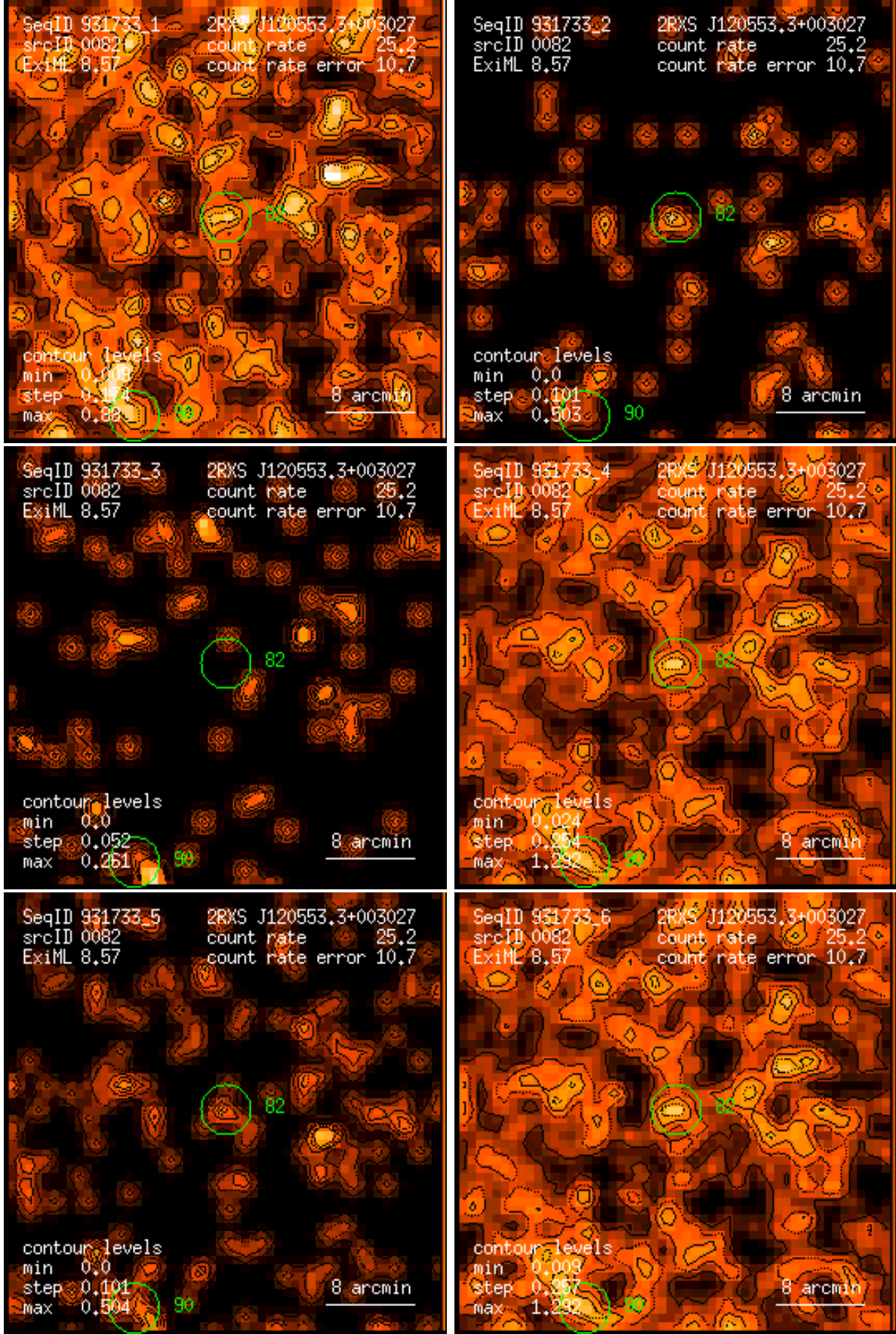
Figure 82: RASS 931733: detection 0082: band rate images, Gaussian filter: (1) PSPC channels 11 – 41, (2) 52 – 90, (3) 91 – 201, (4) 11 – 235, (5) 52 – 201, (6) 11 – 201. Broad band rates in counts/ks. Band rate contour levels in counts/ks/arcmin 2 .
