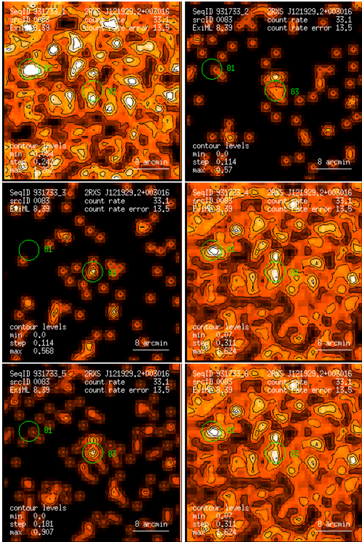
Figure 83: RASS 931733: detection 0083: band rate images, Gaussian filter: (1) PSPC channels 11 – 41, (2) 52 – 90, (3) 91 – 201, (4) 11 – 235, (5) 52 – 201, (6) 11 – 201. Broad band rates in counts/ks. Band rate contour levels in counts/ks/arcmin 2 .
