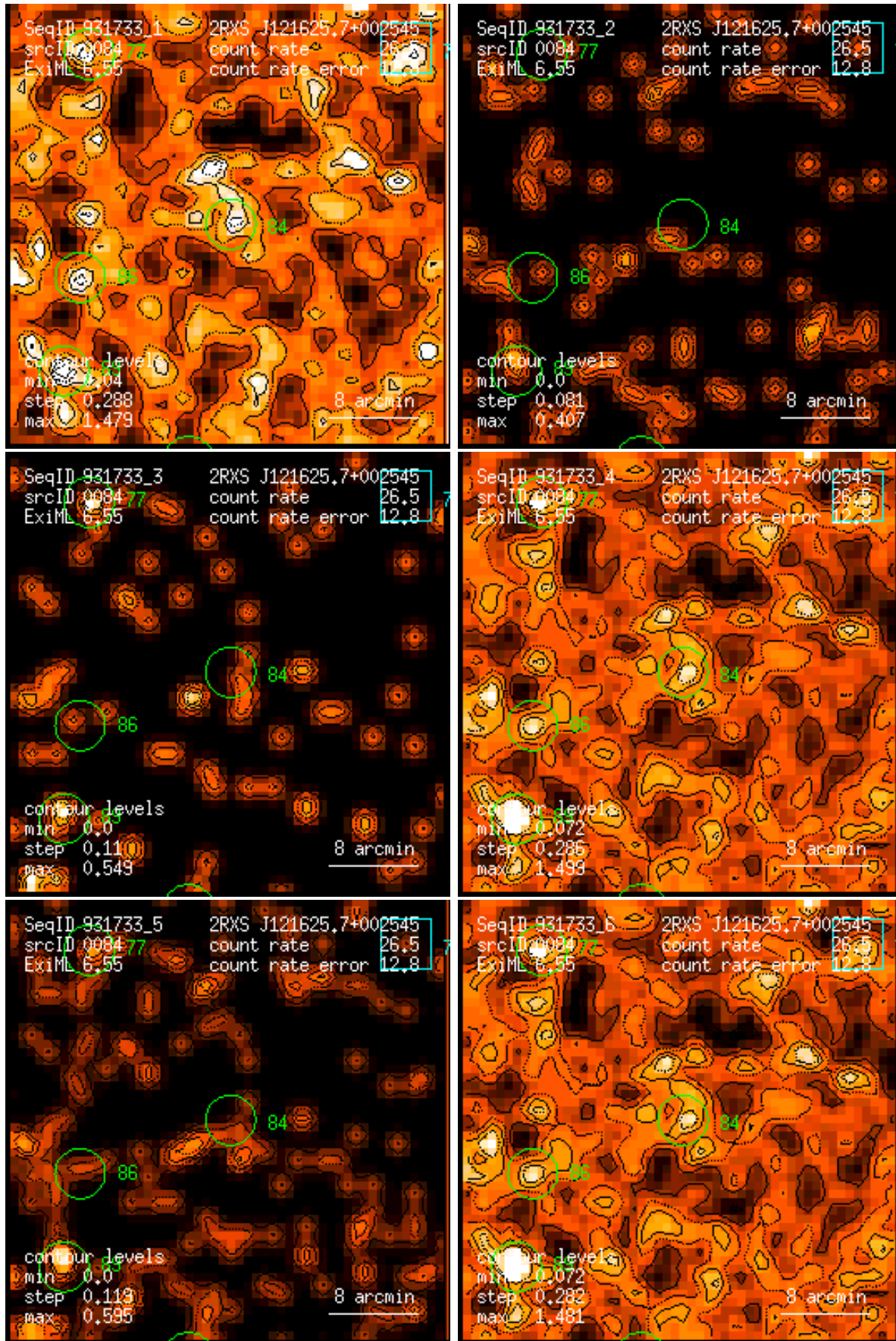
Figure 84: RASS 931733: detection 0084: band rate images, Gaussian filter: (1) PSPC channels 11 – 41, (2) 52 – 90, (3) 91 – 201, (4) 11 – 235, (5) 52 – 201, (6) 11 – 201. Broad band rates in counts/ks. Band rate contour levels in counts/ks/arcmin 2 .
